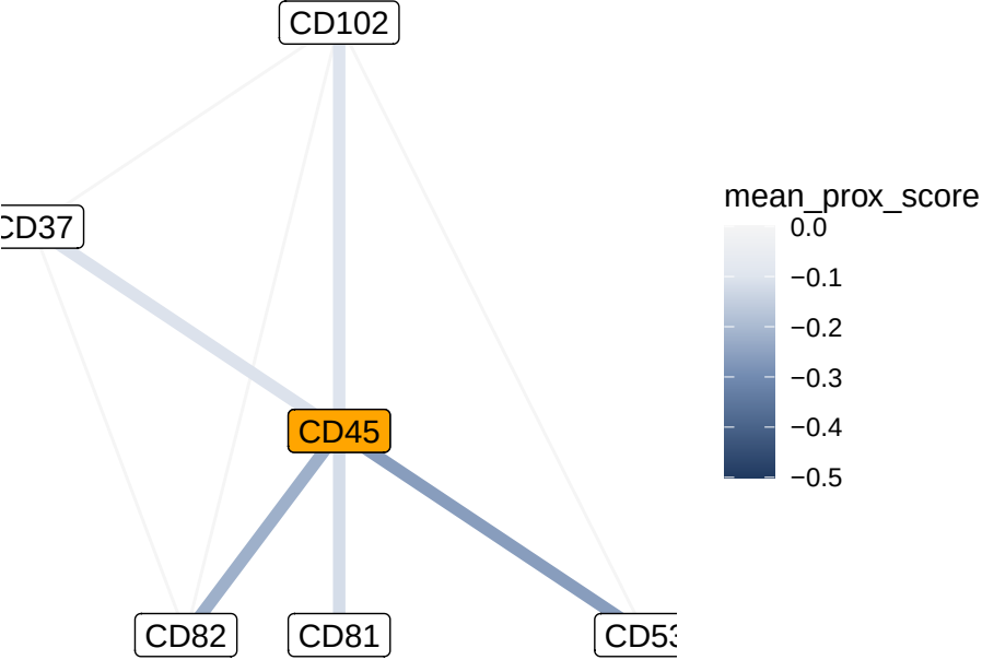
CD45 Interaction Network
