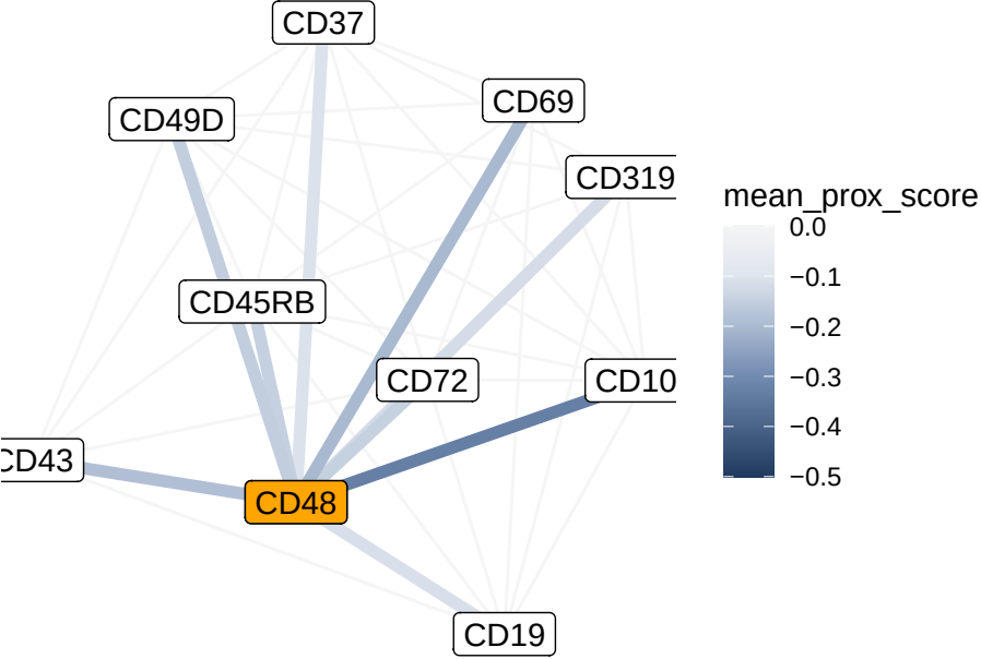
CD48 Interaction Network
