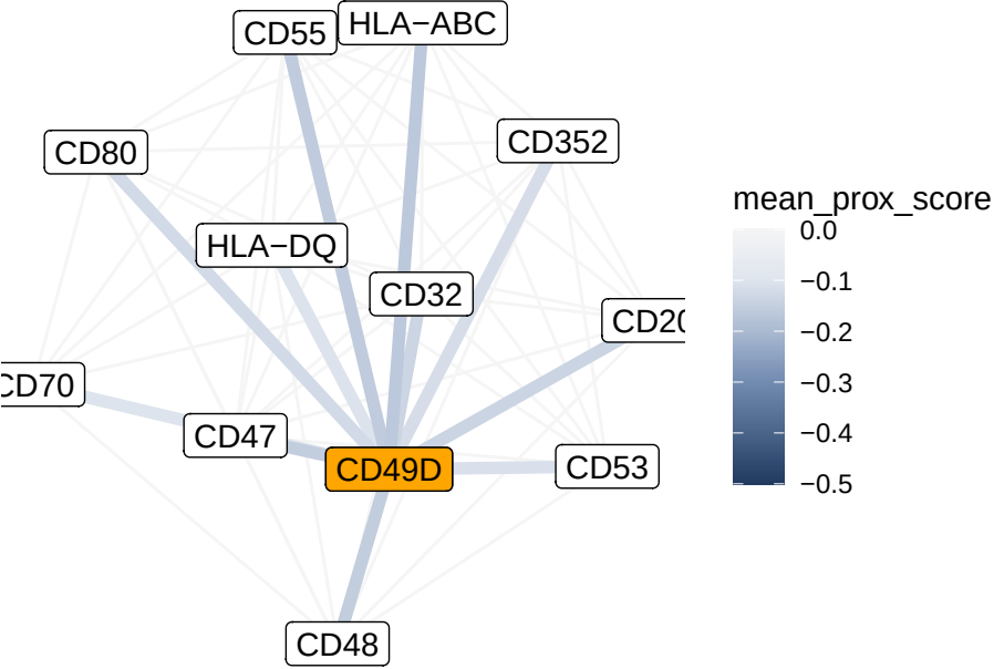
CD49D Interaction Network
