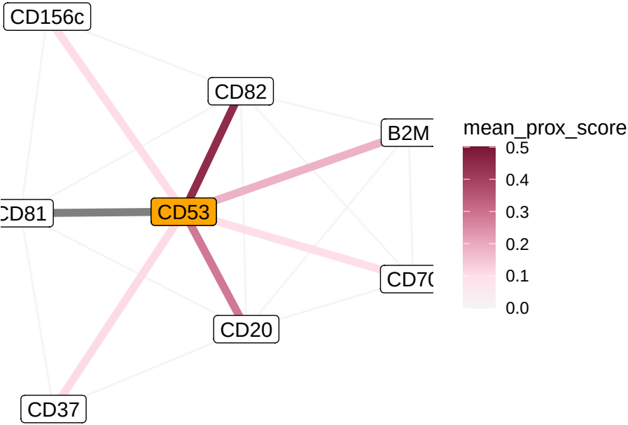
CD53 Interaction Network
