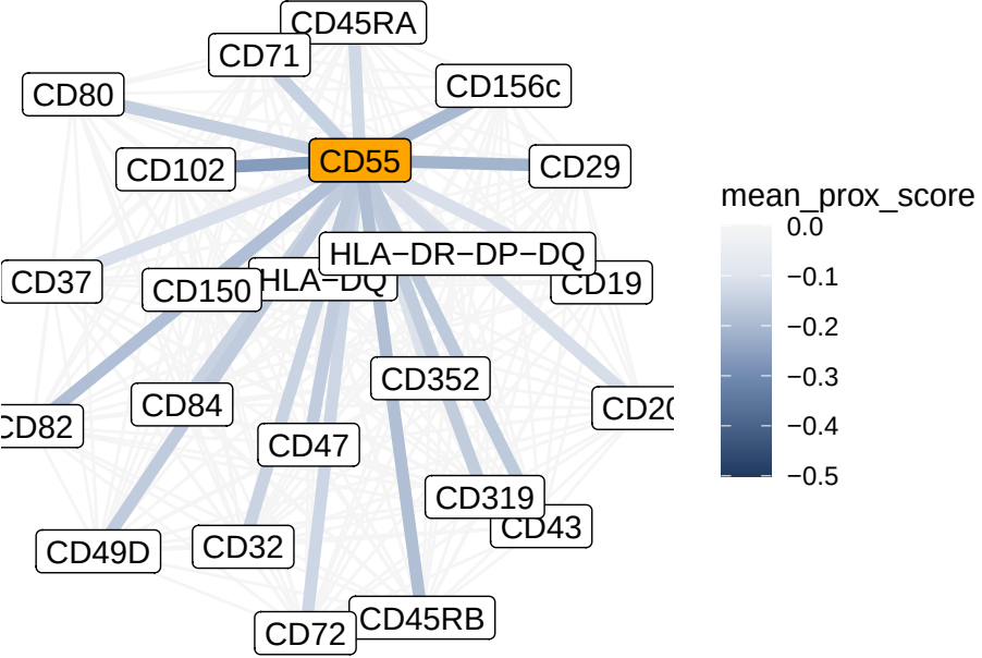
CD55 Interaction Network
