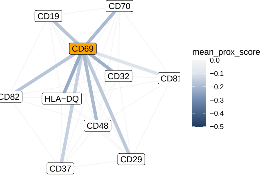
CD69 Interaction Network
