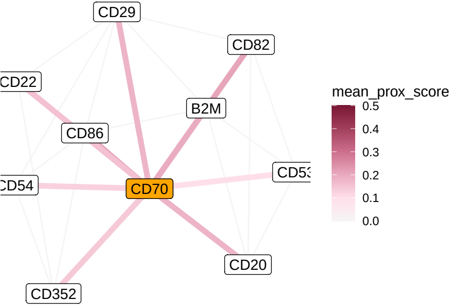
CD70 Interaction Network
