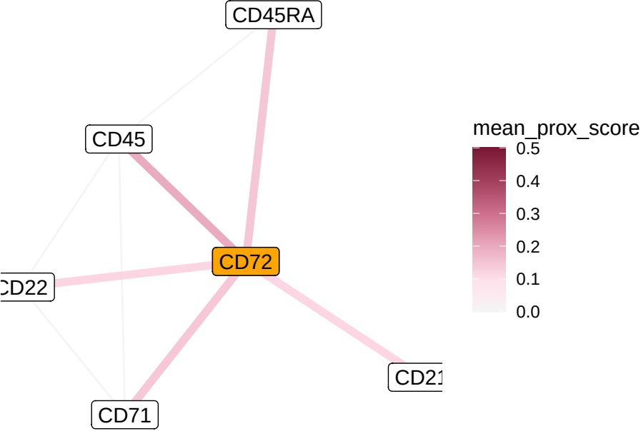
CD72 Interaction Network
