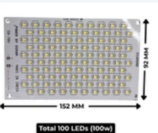
100w (White) Flood Light Plate - High Brightness (Diamond)...
