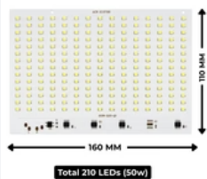
50w Direct On Board pcb without chock
