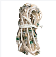
Pixel LED 5inch Gel wire on Rope (Multicolor, WS2811, 50LEDs) 20 Feet Length
