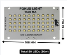
50w (White) Flood Light Plate - High Brightness (Fokus Light )..
