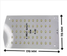
50w (White) Street Light Plate - High Brightness (R-82) 1500Ah..
