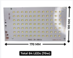
70w (White) Flood Light Plate - High Brightness (AS-60) 750ma...
