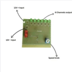
12V 6-Channel Chaser (12V Running Effects ) 100 LED Per...
