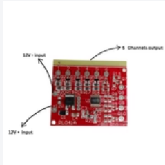
12V 5-Channel Chaser (12V 32 Running Effects ) 500 LED Per...
