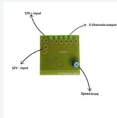
12V 5-Channel Chaser (12V Running Effects ) 100 LED Per...
