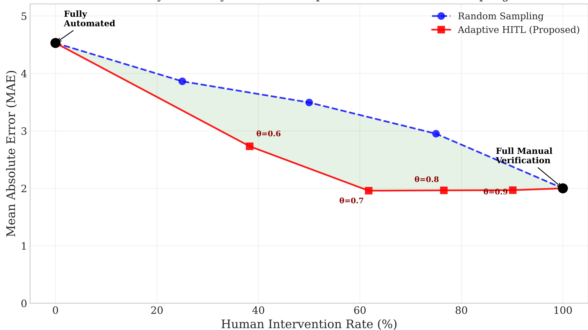
Accuracy-Efficiency Trade-off: Adaptive HITL vs Random Sampling
