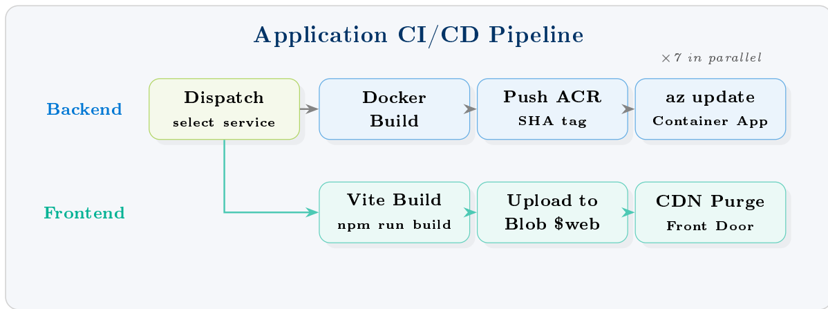
Figure 3: Application pipeline: per-service Docker build, ACR push, Container App update. Frontend uploads to Blob Storage.
