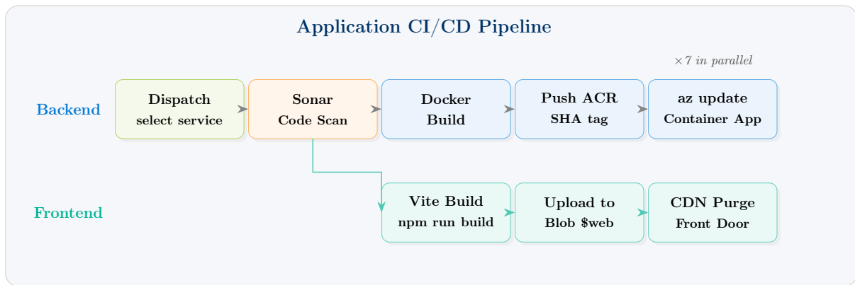
Figure 3: Application pipeline: per-service Docker build, ACR push, Container App update. Sonar code scan runs after dispatch for both Backend and Frontend. Frontend uploads to Blob Storage.
