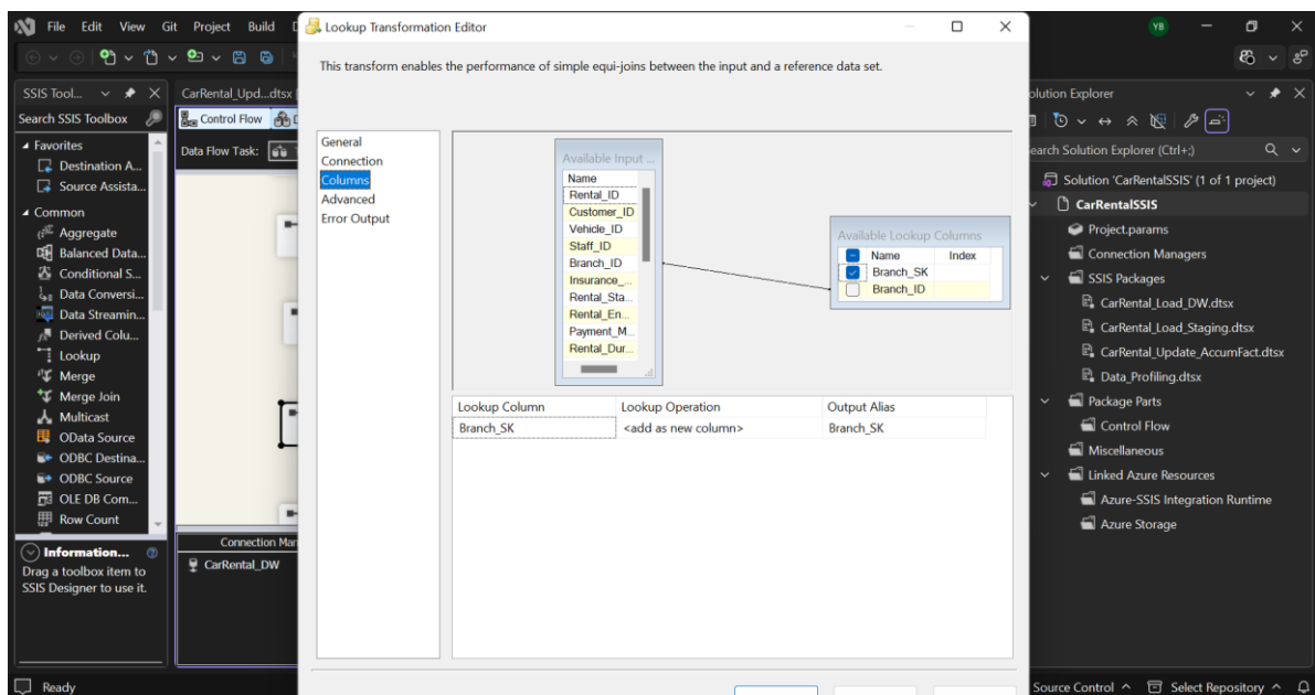
Lookup — DimBranch: showing join on Branch_ID, output Branch_SK
