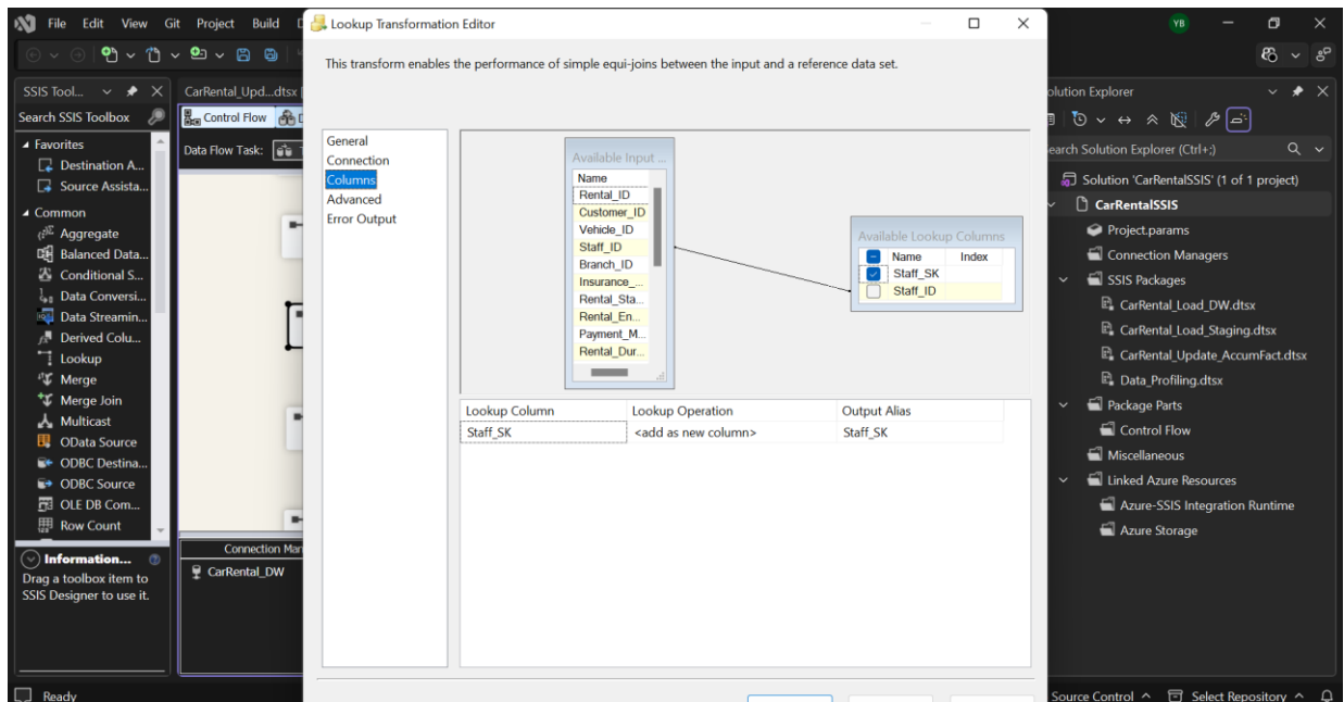
Lookup — DimStaff: showing join on Staff_ID, output Staff_SK
