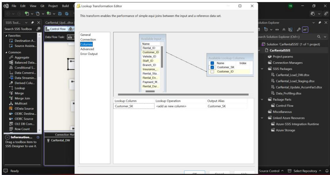
Lookup — DimCustomer: showing join on Customer_ID, output Customer_SK
