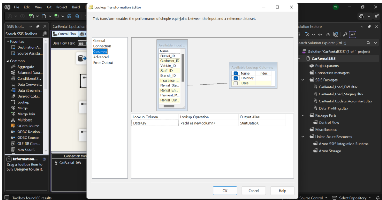
Lookup — DimDate (Start): showing join on Rental_Start_Date, output Start_Date_SK
