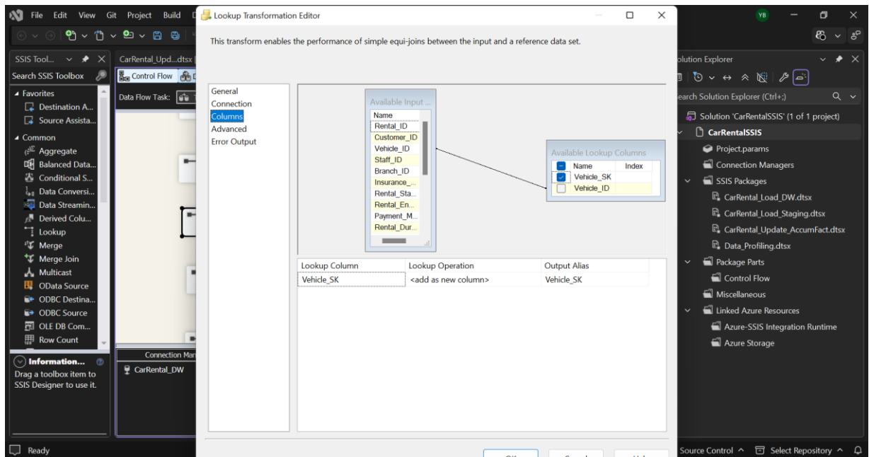
Lookup — DimVehicle: showing join on Vehicle_ID, output Vehicle_SK
