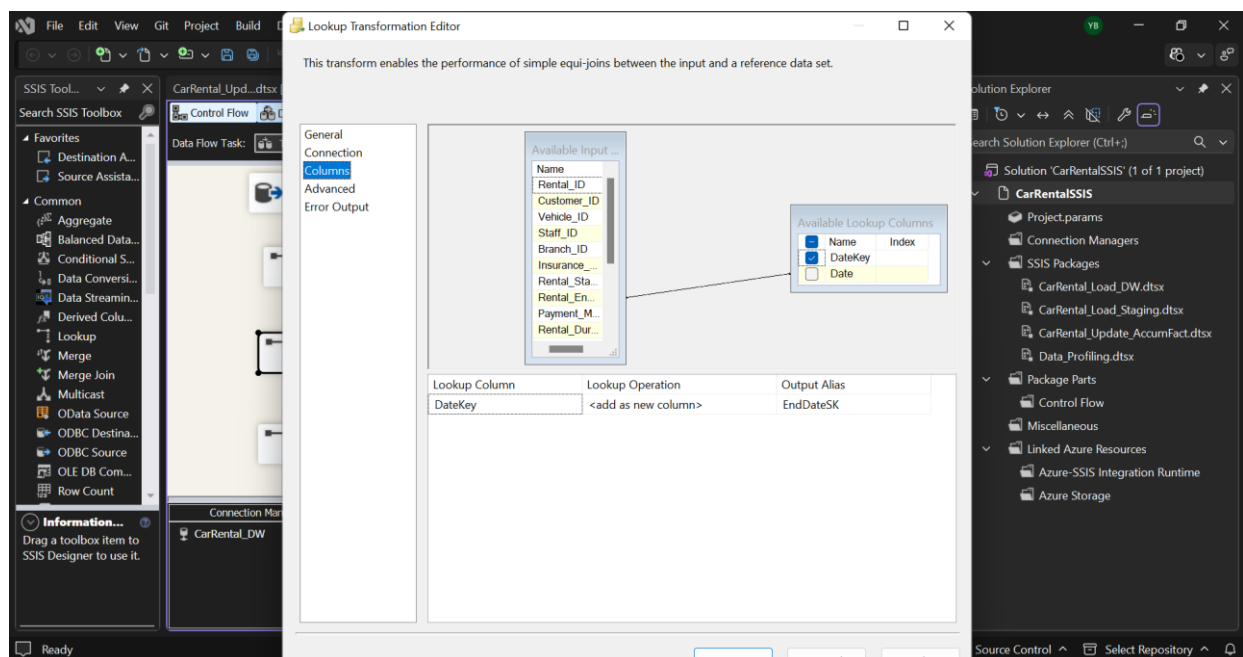
Lookup — DimDate (End): showing join on Rental_End_Date, output End_Date_SK
