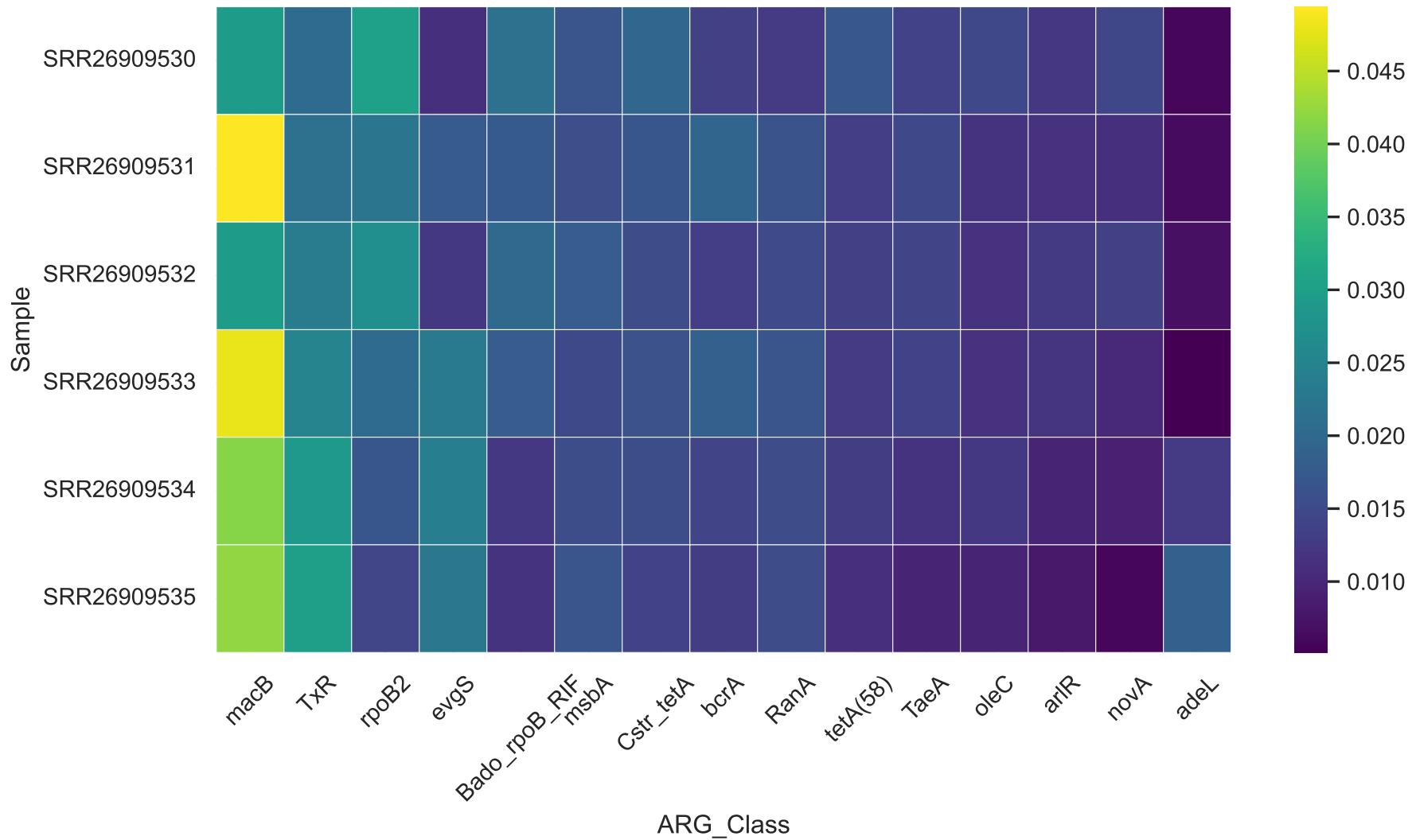
Delhi ARG Profile
