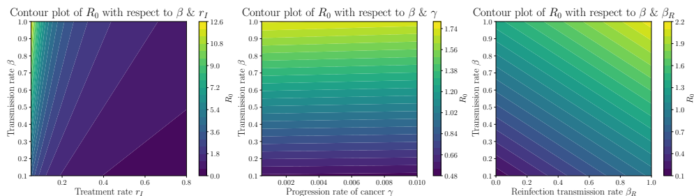
Figure 11: Contour plots of \mathcal{R}_0 with different parameter combinations
