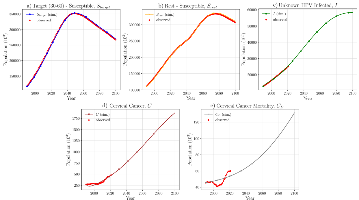
Figure 2: Comparison of Actual values vs. Simulation Prediction for compartments: a) S_{Target} , b) S_{Rest} , c) I , d) C and e) C_D .
