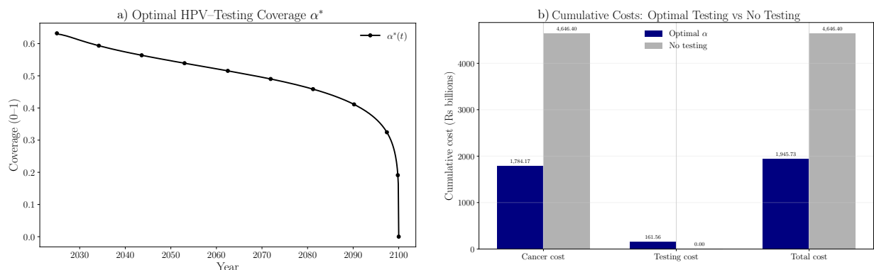
Figure 7: Panel (a): Optimal time-varying HPV-testing coverage \alpha^*(t) beginning in 2025. Panel (b): Cumulative cervical-cancer treatment cost, HPV-testing cost, and their sum (2025-2100) under the optimal policy (navy) versus a no-testing baseline (grey), highlighting the economic impact achieved by the optimal policy.
