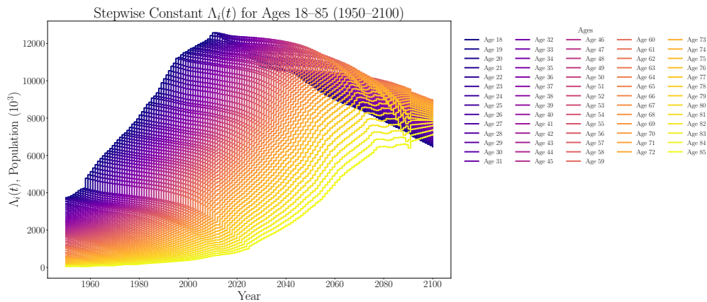
Figure 9: Piecewise/Step-wise constant functions \Lambda_i(t) for females of ages i = 18, \dots, 85 in India (1950–2100)
