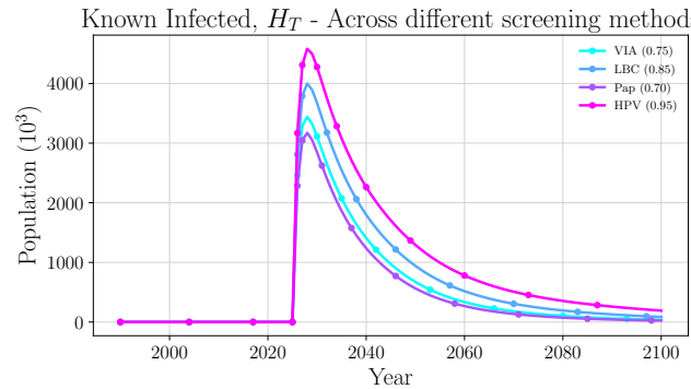
Figure 10: Modelled number of HPV-tested positive Infected women ( H_T ) under four screening tests with increasing test sensitivity H^+ : Pap cytology (0.70), VIA (0.75), LBC (0.85) and HPV DNA testing (0.95). Higher sensitivity translates into substantially more infections detected.
