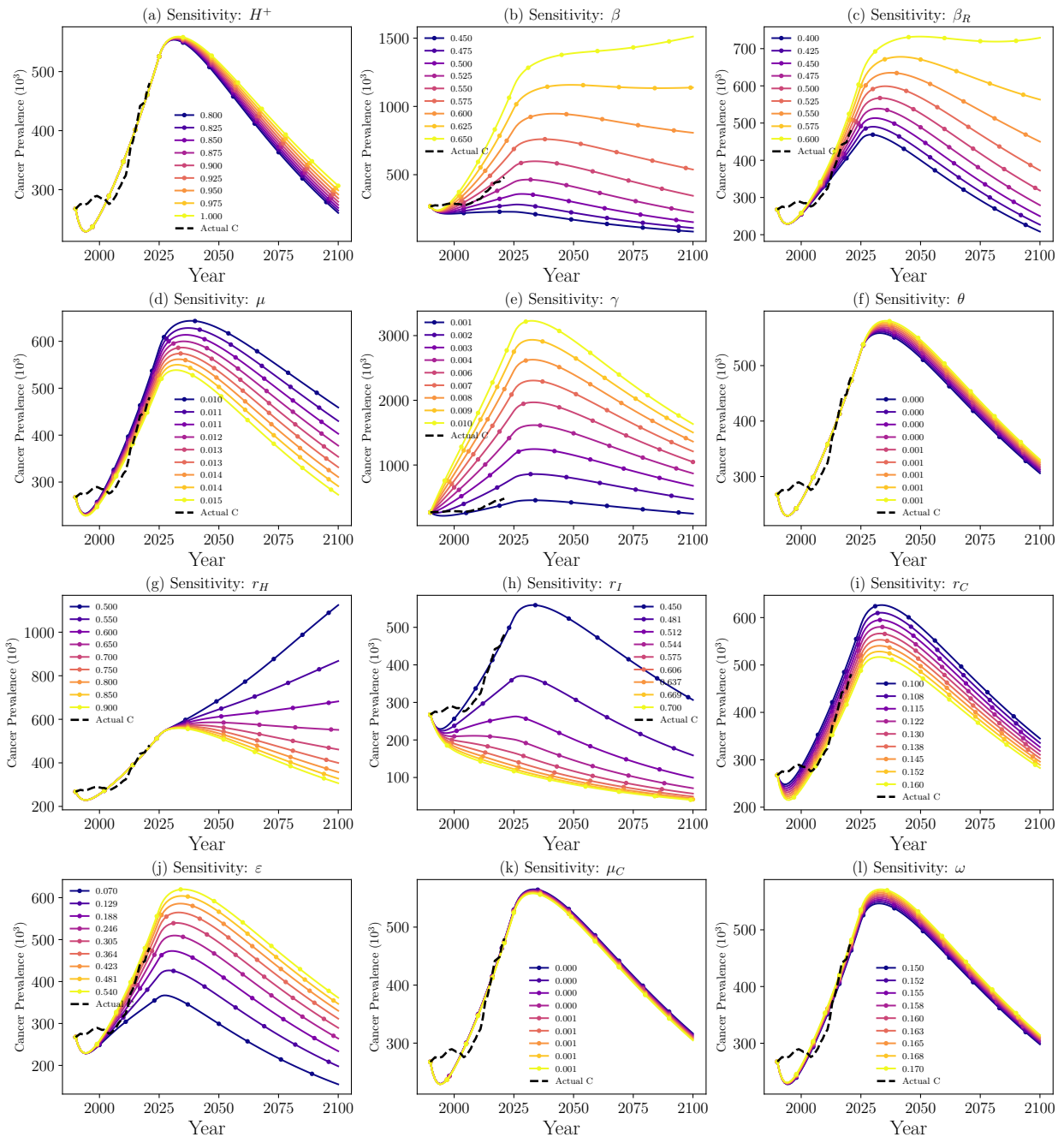
Figure 3: Sensitivity Analysis of Model Parameters (With 90% Testing Coverage)
