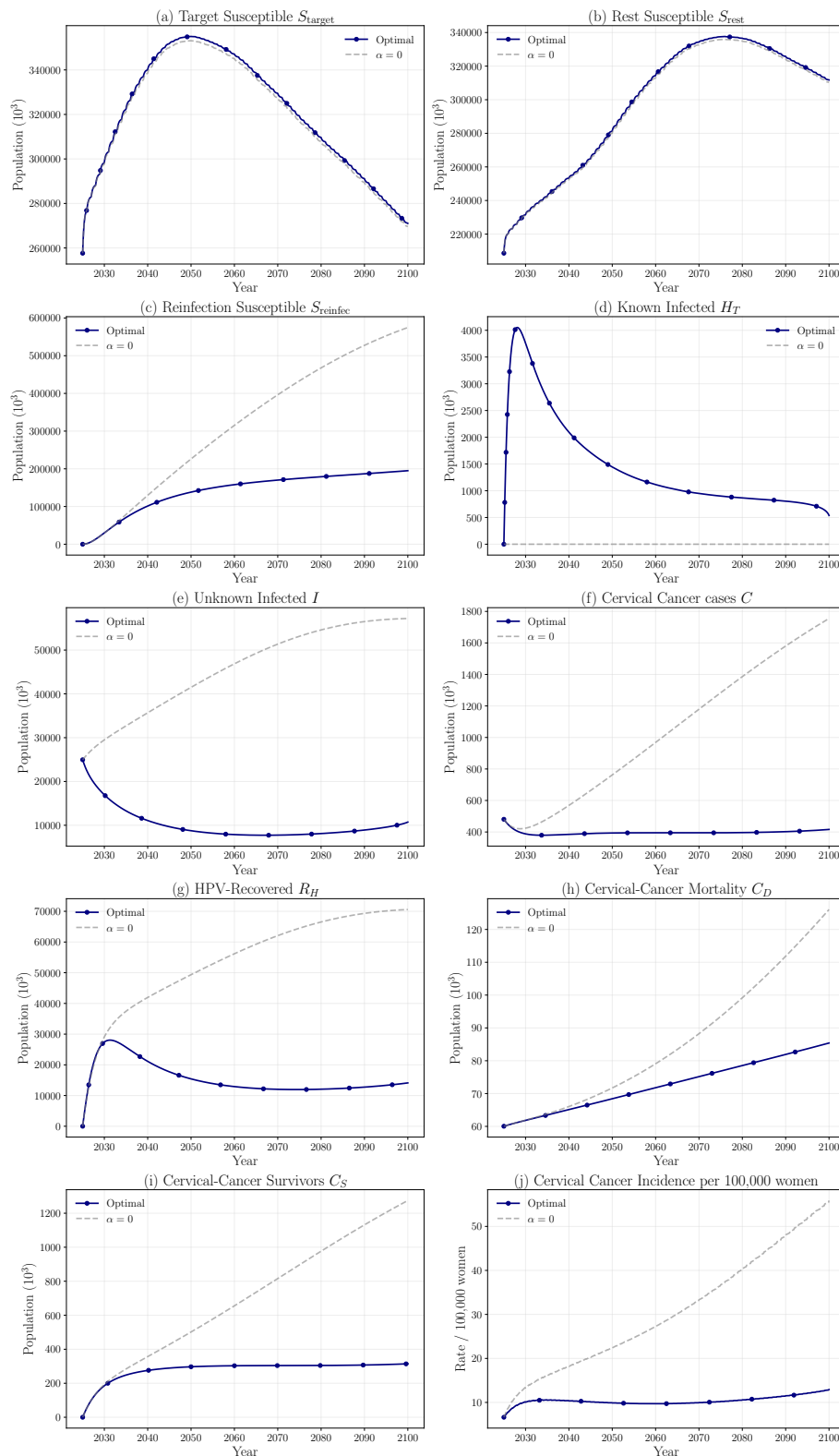
Figure 8: Dynamic HPV-testing policy obtained from optimal-control analysis (solid navy) versus the natural-history baseline with no testing (grey dashed), simulated from 2025 to 2100. Screening is restricted to women aged 30–60, and the coverage \alpha^*(t) is chosen to minimise the weighted sum of testing effort and cervical-cancer treatment costs. Panels (a)-(i) show the trajectories for nine state variables, and panel (j) shows annual cervical-cancer incidence per 100 000 women.
