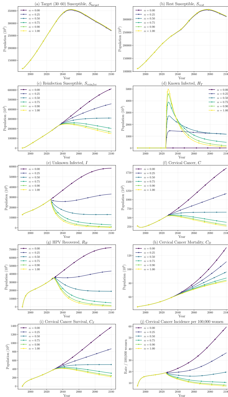
Figure 4: Effect of HPV Testing Rate \alpha , on on nine state variables (a)-(i) and Cervical-Cancer Incidence per 100K women (j)
