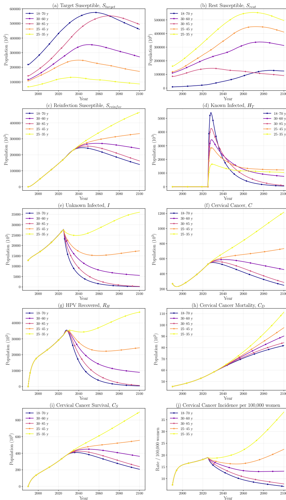
Figure 5: Effect of choosing different Target Age Groups for Testing, on all nine state variables (a)-(i) and on Cervical Cancer Incidence per 100K women (j) (With 65% Testing Coverage)
