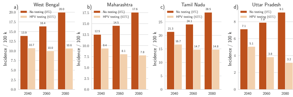
Figure 6: Projected Cervical Cancer Incidence per 100,000 women in four Indian states: a) West Bengal, b) Maharashtra, c) Tamil Nadu, d) Uttar Pradesh, under two screening scenarios: Baseline (0%) vs HPV Testing (65%). Incidence is shown for the years 2040, 2060, and 2080. Simulations use state-specific parameters and initial conditions calibrated to 2011 data.
