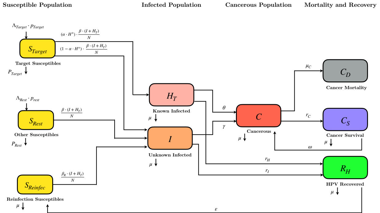
Figure 1: Compartmental Model for HPV and Cervical Cancer Dynamics with Age-Specific HPV Testing
