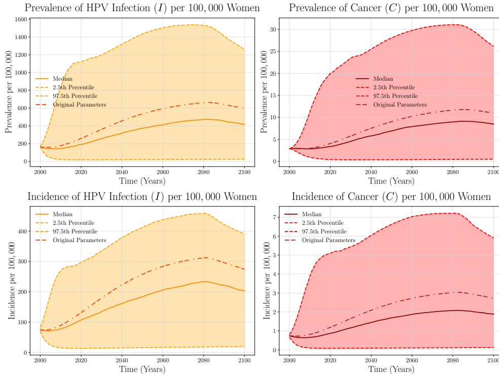
Figure 12: Monte Carlo Parameter Sampling Analysis. Shaded regions denote the 2.5th to 97.5th percentile bounds across 1000 simulations. The solid curves represent the median projections, and the red curves correspond to the simulation using the original parameter set. The left panels (orange shades) pertain to HPV infection outcomes, while the right panels (red shades) pertain to cancer outcomes.
