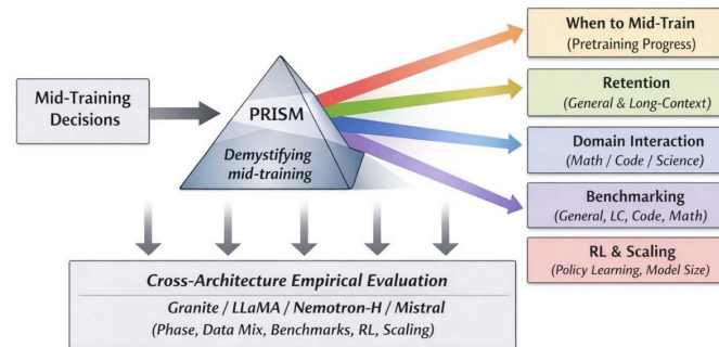
Figure 1 PRISM overview. Mid-training decisions are decomposed into their principal design axes, including retention of general and long-context abilities, domain interaction (math, code, science), benchmark selection, reinforcement learning compatibility, and scaling behavior. PRISM enables holistic evaluation of mid-training choices across model families at scale.
