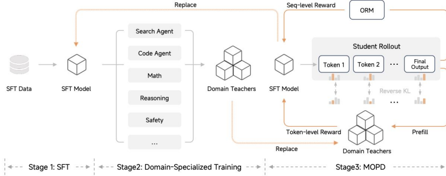
Figure 3 Overview of MiMo-V2-Flash post-training stages.
