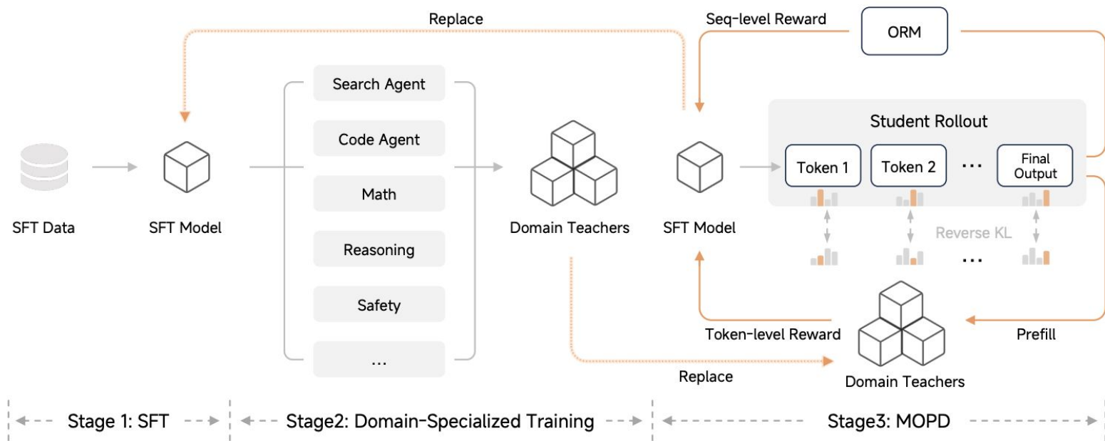
Figure 3 Overview of MiMo-V2-Flash post-training stages.
