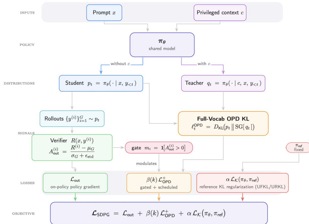
Figure 1: Overview of the Self-Distilled Policy Gradient (SDPG) objective, combining rollout-based outcome optimization, gated On-Policy Distillation (OPD) from privileged context, and a KL regularization to a fixed reference policy. Note that OPD is also a form of policy gradient.
