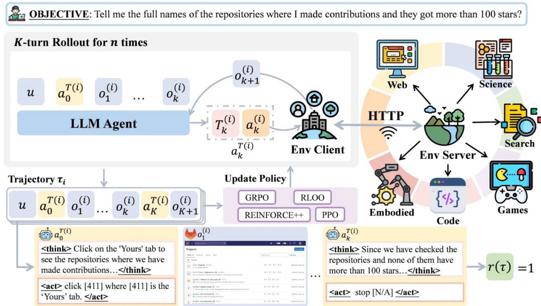
Figure 2 Overview of the AgentGym-RL framework. It features a decoupled, flexible, and extensible architecture, comprising three primary modules—the environment, the agent, and the training module. It supports diverse scenarios, environments, and algorithms.
