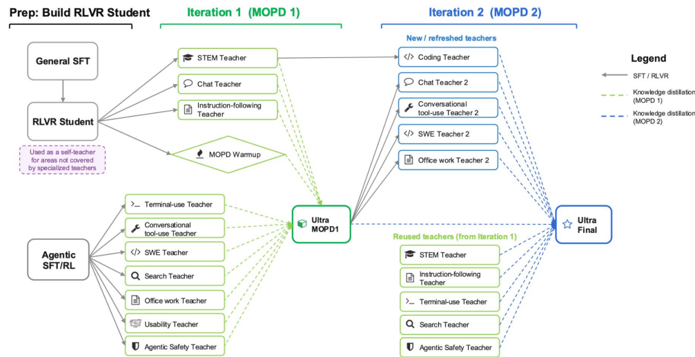
Figure 10 | Two-iteration MOPD training pipeline for Nemotron 3 Ultra. Iteration 1 distills signals from general and agentic teachers into Ultra MOPD1. Iteration 2 initializes additional teachers from Ultra MOPD1, reuses first-round teachers, and distills all resulting signals into Ultra Final. RLVR Student also serves as a self-teacher for areas not covered by specialized teachers.
