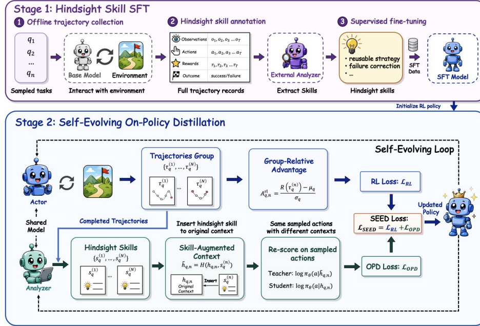
Figure 2: Overview of SEED. Stage 1 (Hindsight Skill SFT) equips the policy to extract hindsight skills from completed trajectories. Stage 2 (Self-Evolving On-Policy Distillation) jointly optimizes outcome-based RL and skill-conditioned OPD in a self-evolving agentic loop.
