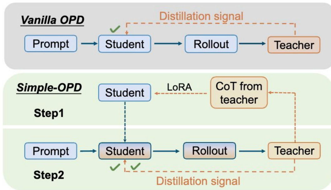
Figure 1: Overview of vanilla OPD and Simple-OPD. Simple-OPD first warms up the student with teacher-generated CoT using LoRA, followed by standard OPD.
