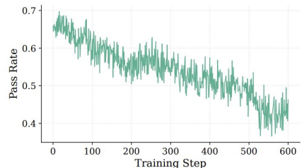
Figure 6 | Batch-wise pass rates across the RL curriculum.
