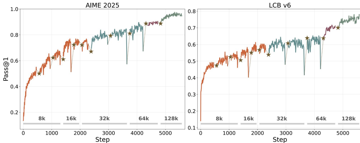
Figure 15. Performance on AIME 2025 (left) and a hard subset of LiveCodeBench v6 (right) during our STEM climb. Self-distillation is indicated through ★ markers; different pre- and mid-trained model versions are shown in different colors. Maximum output length throughout training is indicated at the bottom. Self-distillation is an effective way of resetting numerics after a collapse (visible through sudden drops in performance) and changing the base policy during our run. As we made infrastructure and algorithmic improvements throughout our climb, self-distillation because of run collapses became less frequent.
