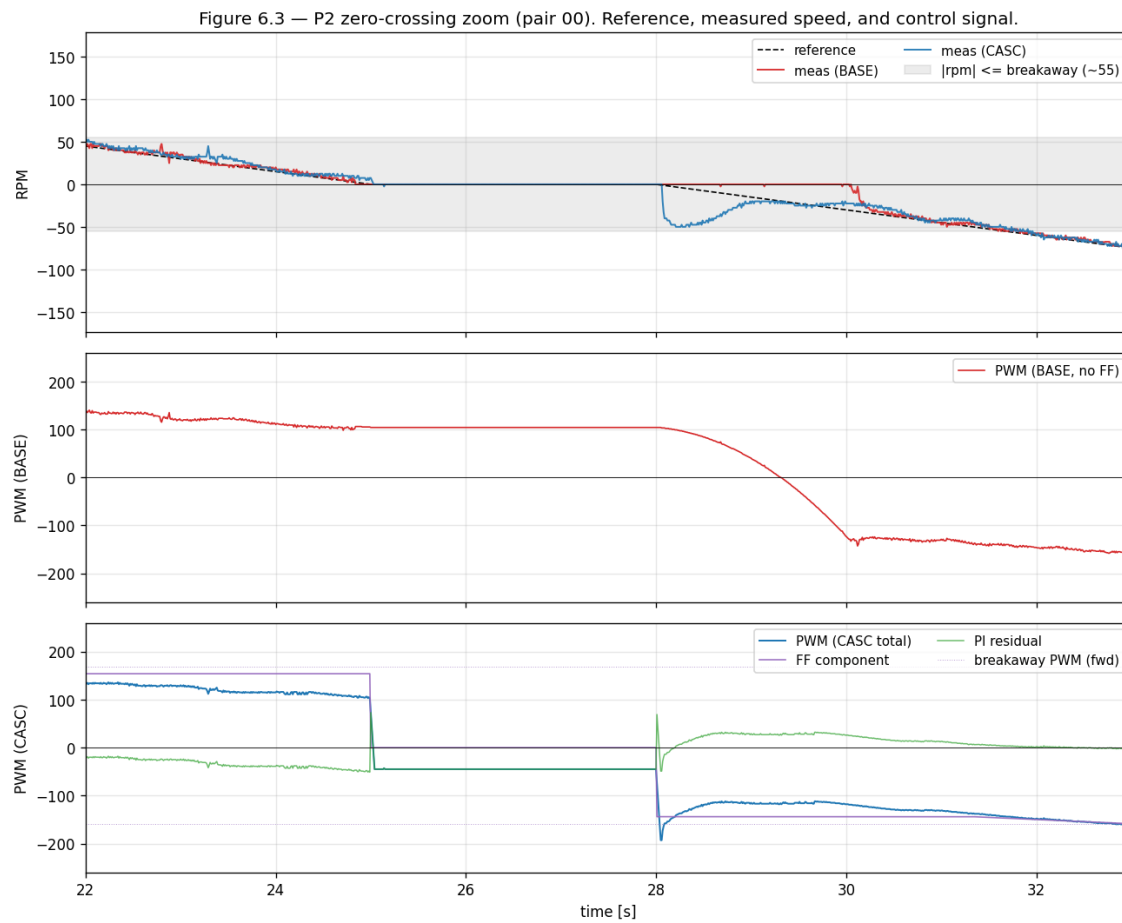
FIGURE 6.3: P2 zero-crossing zoom (pair 00) showing the mechanism behind the cascade penalty on P2. Top: reference and measured RPM for BASE (red) and CASC (blue). Middle: BASE PWM—smooth, monotone through the deadzone. Bottom: CASC PWM decomposed into FF component (purple) and PI residual (green), with the breakaway PWM levels marked as dotted lines. The FF jumps at t \approx 25 s (entering the deadzone) and t \approx 28 s (re-emerging in reverse) are direct injections of step-like PWM into a slow-ramp tracking task; the second jump produces a \approx 55 rpm reverse overshoot that BASE does not exhibit.
