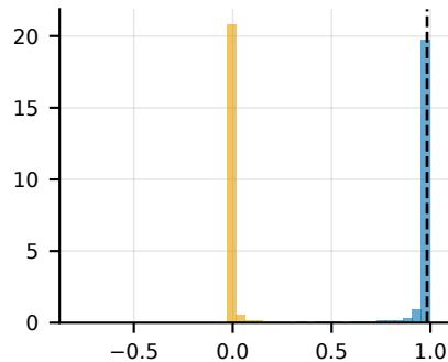
CIFAR-10, BPP 10% (AUROC 0.871)
