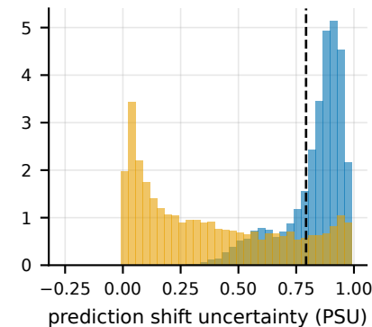
CIFAR-10, BPP 10% (AUROC 0.871)
