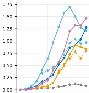
CIFAR-100
