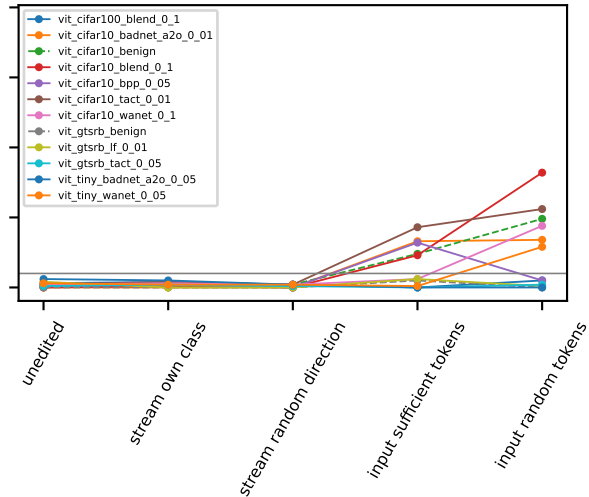
non flagged images, flag rate at q 0.05
