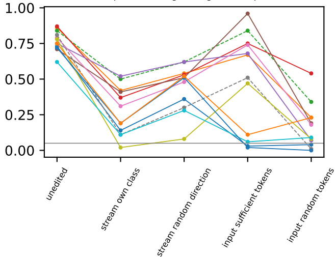
false positive images, flag rate at q 0.05
