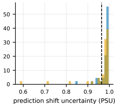
Tiny ImageNet, TaCT 1% (AUROC 0.575)
