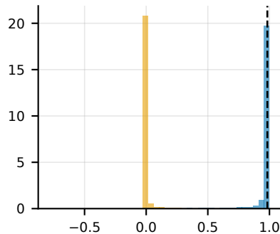
Tiny ImageNet, TaCT 1% (AUROC 0.575)
