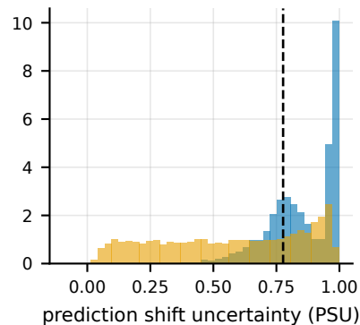
CIFAR-10, BPP 5% (AUROC 0.801)
