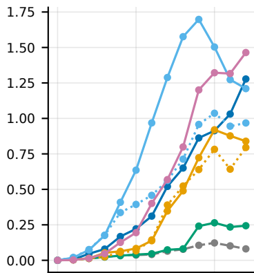
CIFAR-100
