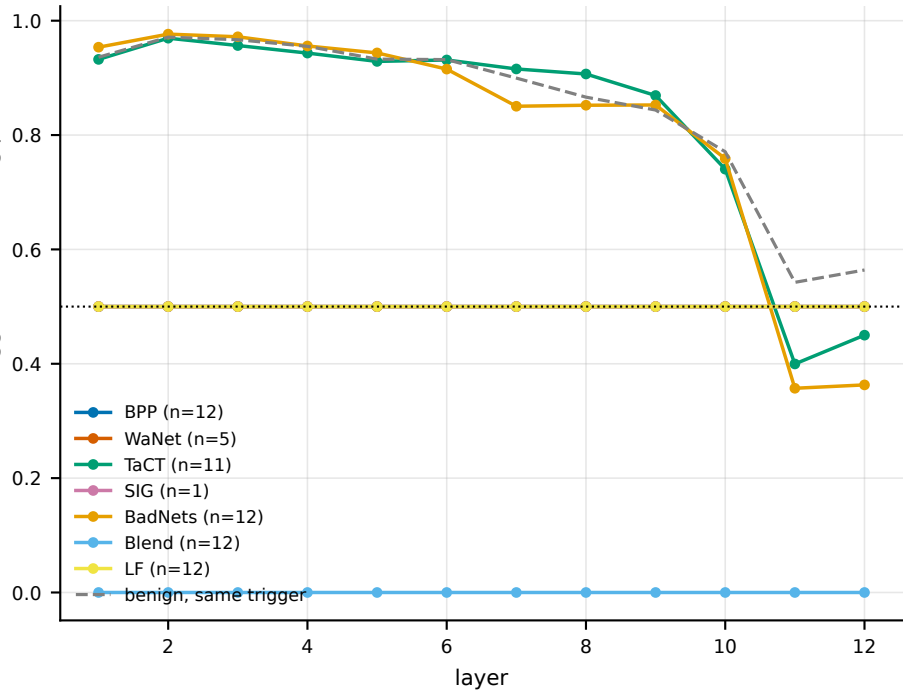
norm rank of the trigger tokens among patches
