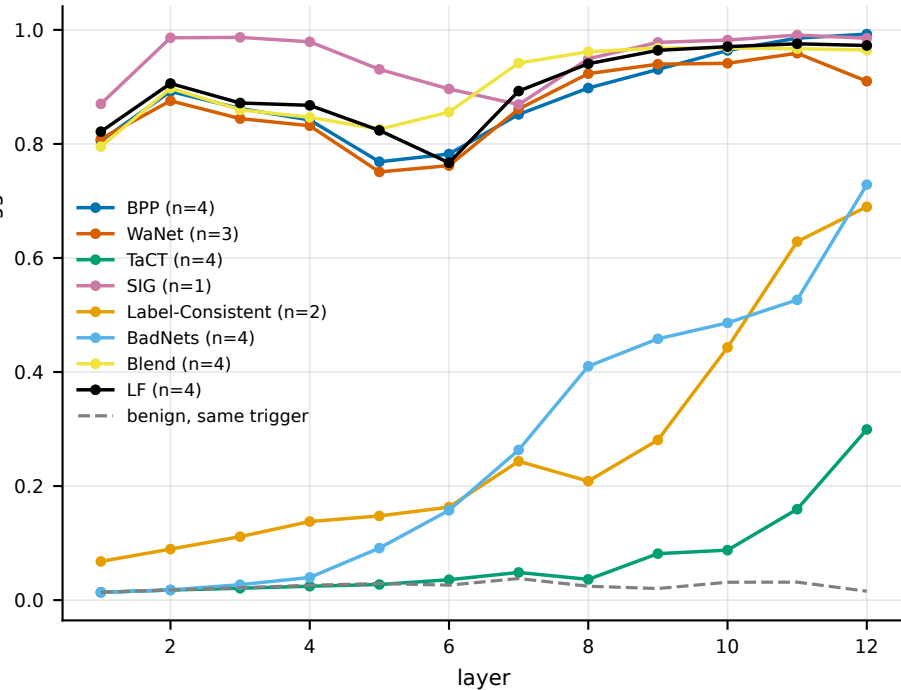
CLS attention mass on the trigger tokens
