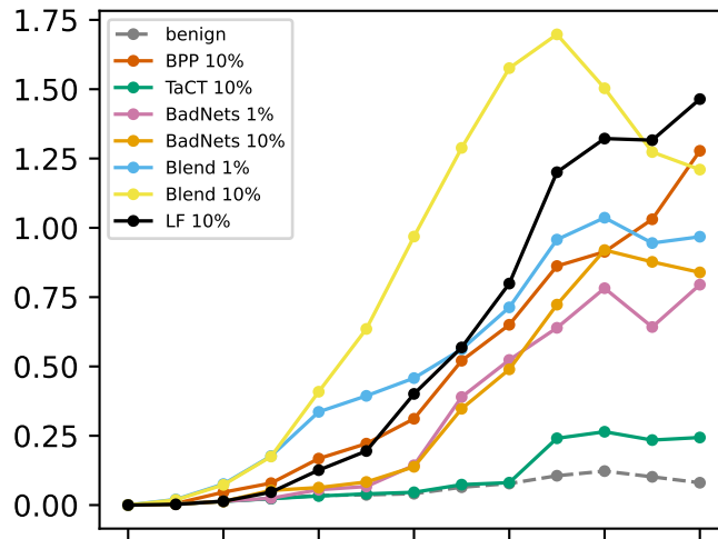
CIFAR-100
