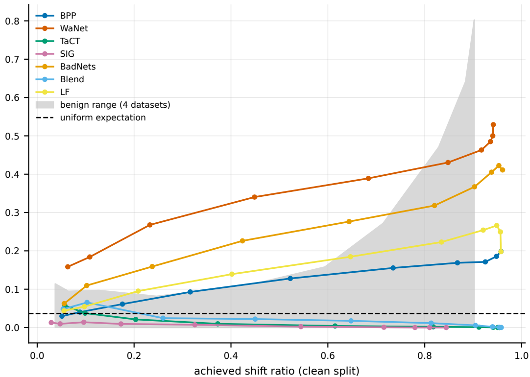
target-class share of shifted clean predictions
