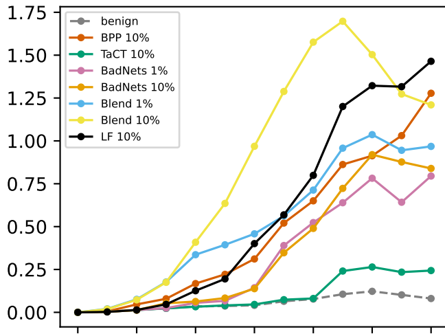
CIFAR-100
