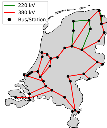
Figure 1: Aggregated power system 2035
