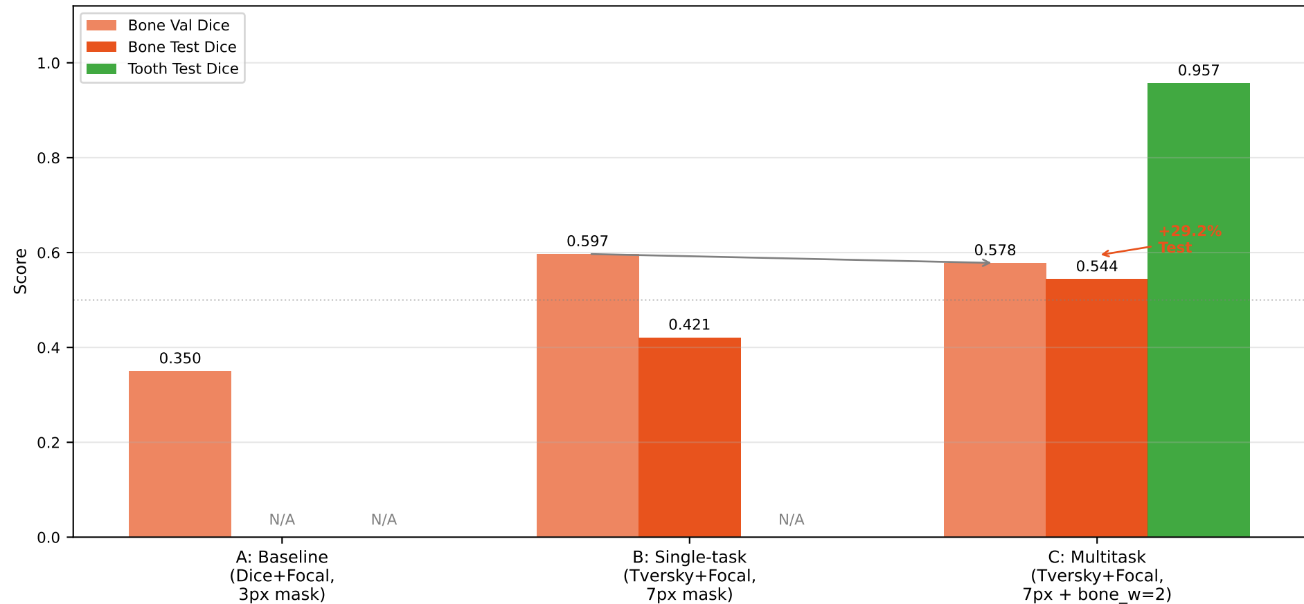
Figure A1 — Ablation Study: Impact of Design Choices on Bone Segmentation
