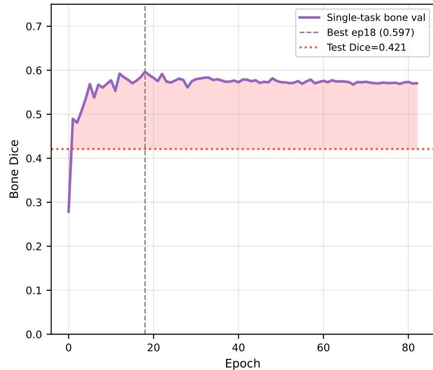
B. Single-task bone_seg — Bone Dice (large train-test gap)
