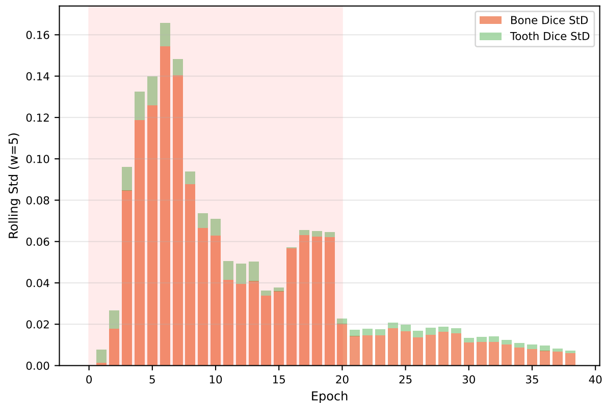
B. Training Instability by Epoch (lower = more stable)
