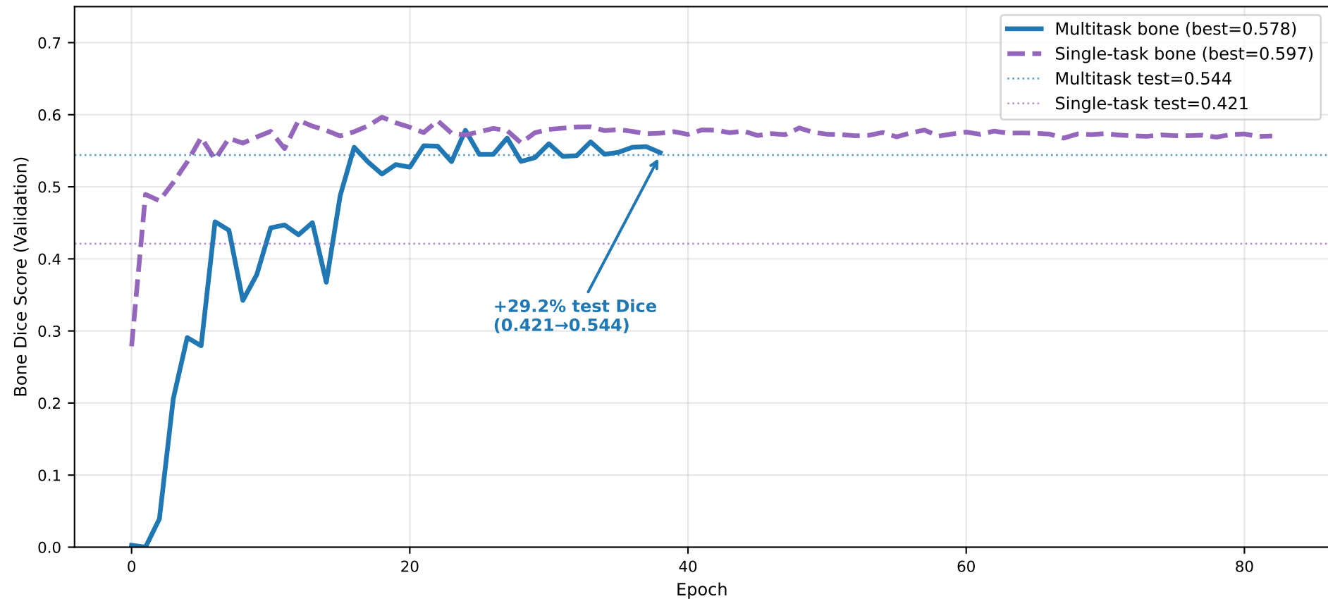
Figure A6 — Multitask vs Single-task Bone Segmentation Learning Curves Multitask achieves +29.2% test improvement with 53% fewer epochs
