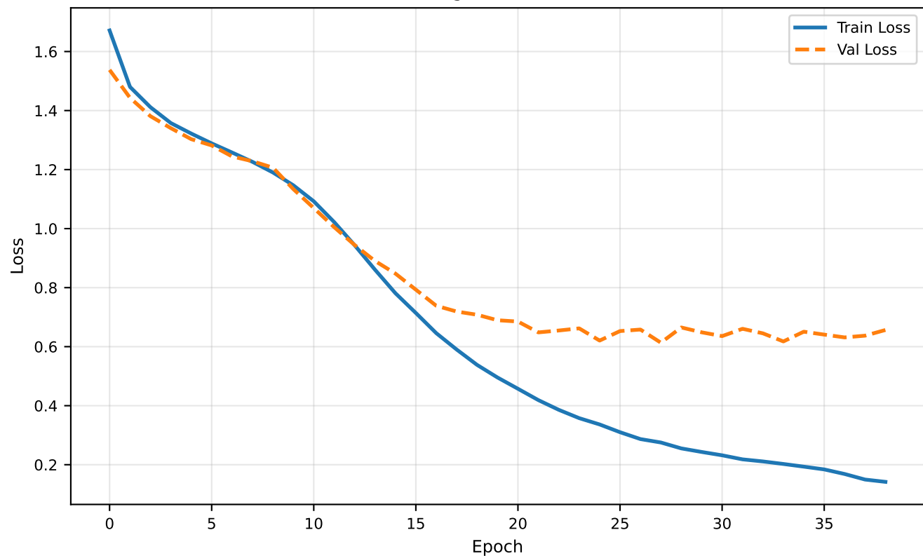
B. Training & Validation Loss
