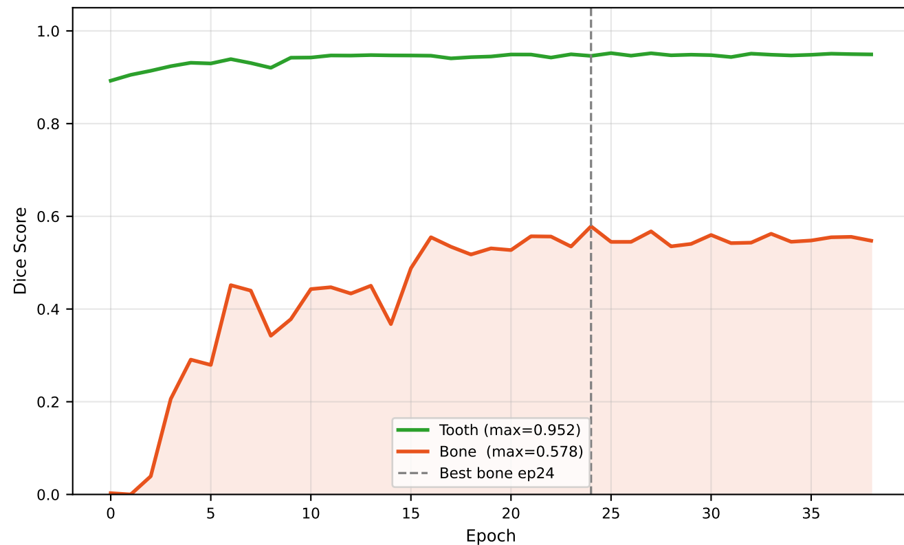
A. Validation Dice Scores
