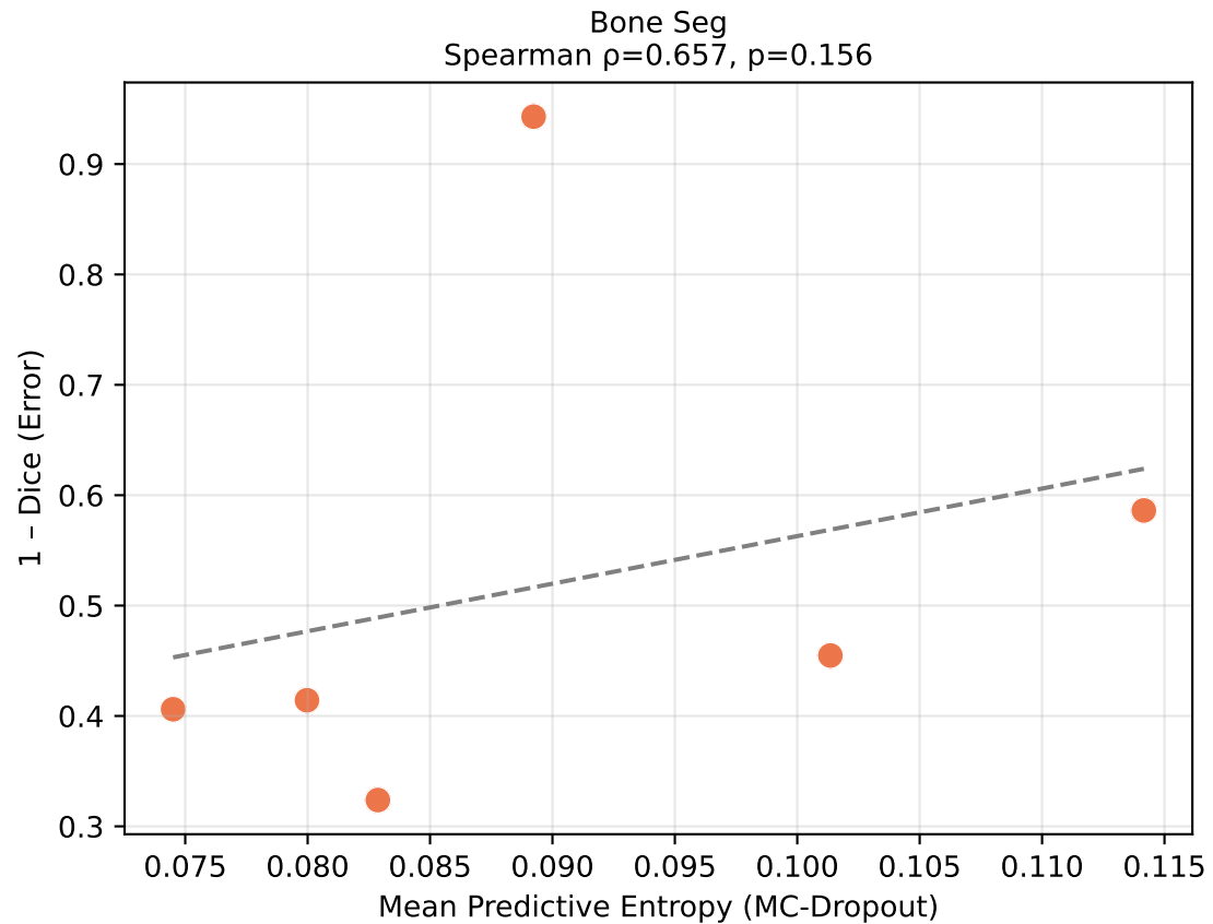
Figure 6 — Uncertainty vs Segmentation Error (Test Subset)
