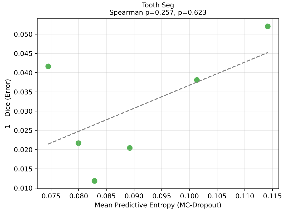
Figure 6 — Uncertainty vs Segmentation Error (Test Subset)
