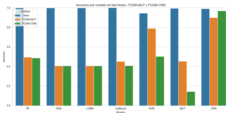
Figura 2.56. Accuracy-FGSM-IOT-23
