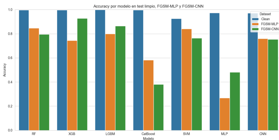
Figura 2.62. Accuracy-FGSM-TON-IOT
