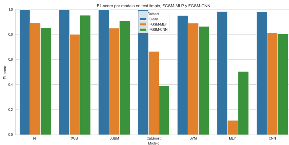
Figura 2.61. F1-FGSM-TON-IOT
