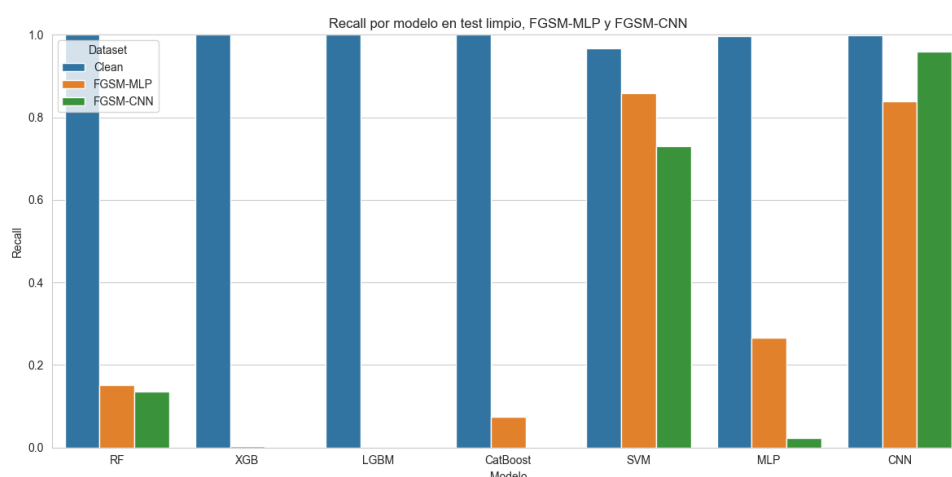
Figura 2.57. Recall-FGSM-IOT-23
