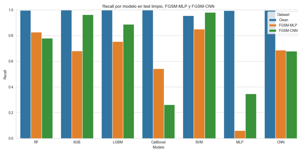
Figura 2.63. Recall-FGSM-TON-IOT
