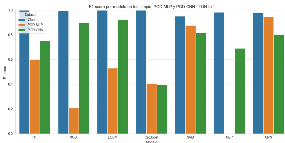
Figura 70. F1-PGD-TON-IOT
