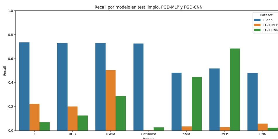
Figura 60. Recall-PGD-UNSW-NB15
