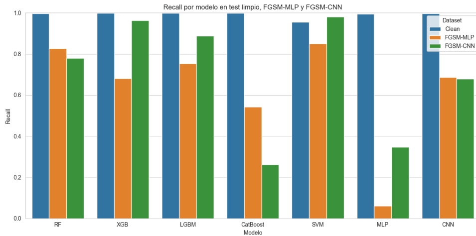
Figura 75. Recall-FGSM-TON-IOT
