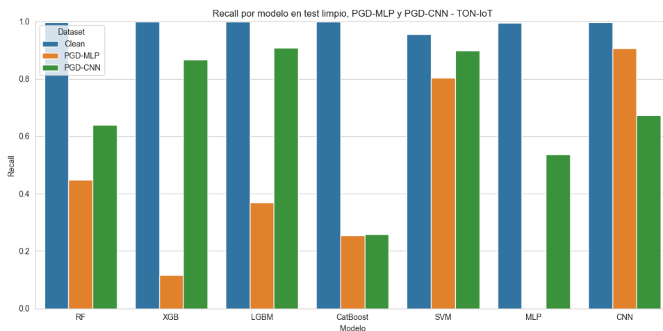
Figura 72. Recall-PGD-TON-IOT
