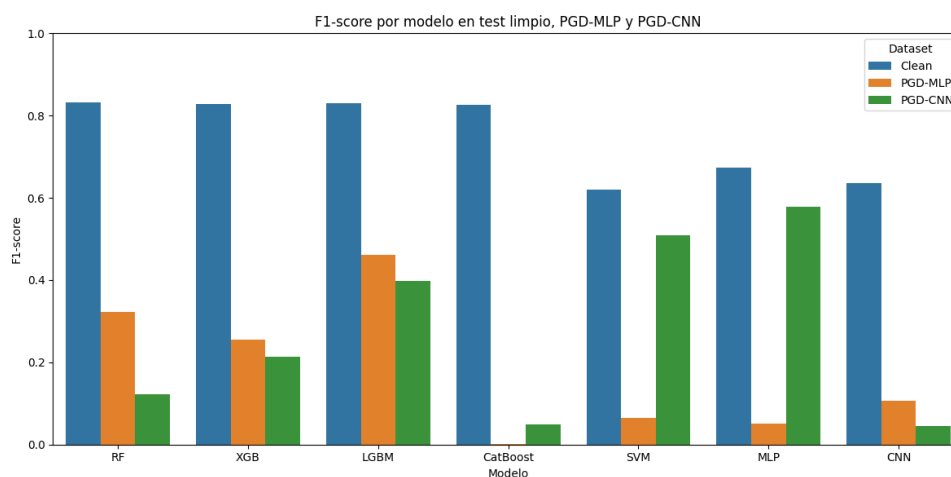
Figura 58. F1-PGD-UNSW-NB15
