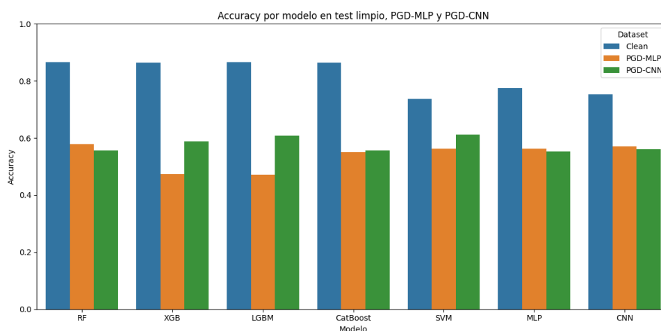
Figura 59. Accuracy-PGD-UNSW-NB15
