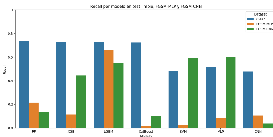
Figura 63. Recall-FGSM-UNSW-NB15
