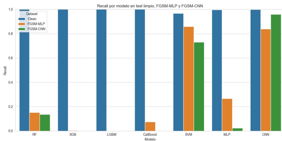
Figura 69. Recall-FGSM-IOT-23
