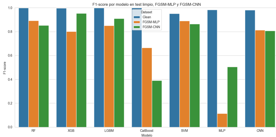
Figura 73. F1-FGSM-TON-IOT
