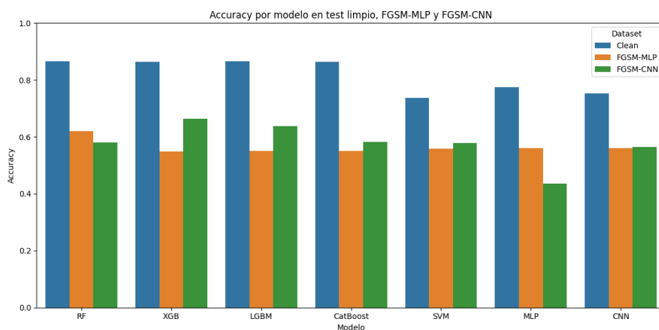
Figura 62. Accuracy-FGSM-UNSW-NB15
