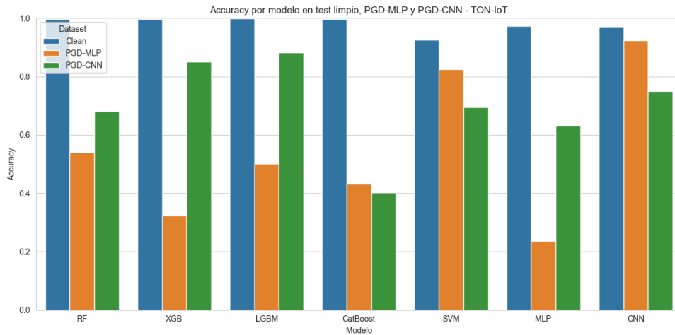
Figura 71. Accuracy-PGD-TON-IOT
