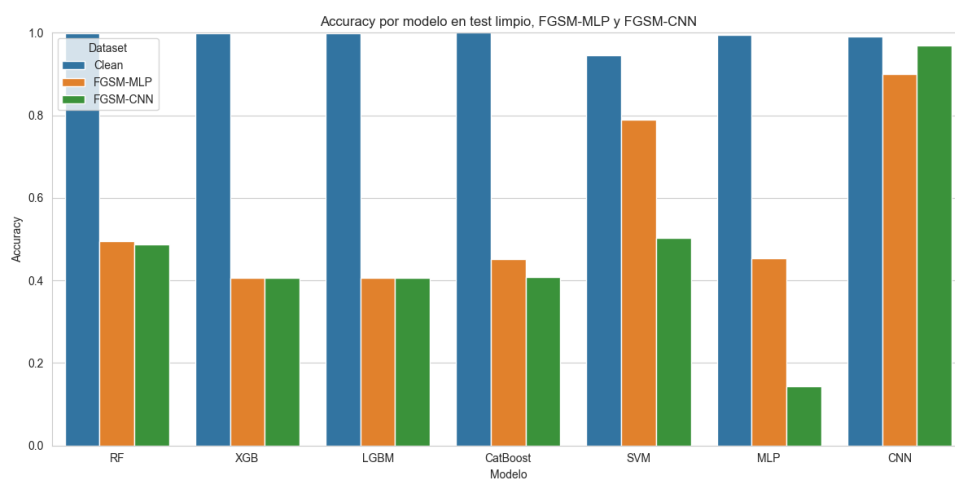
Figura 68. Accuracy-FGSM-IOT-23
