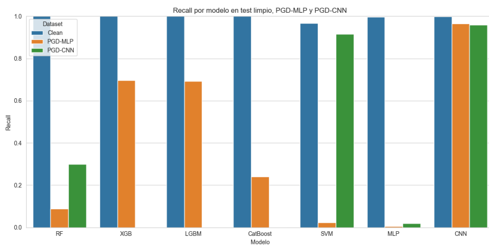
Figura 66. Recall-PGD-IOT-23
