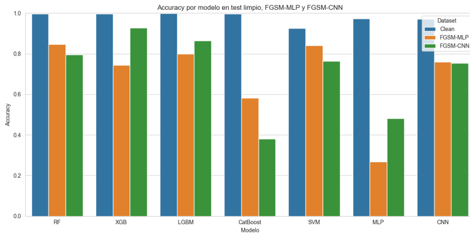
Figura 74. Accuracy-FGSM-TON-IOT
