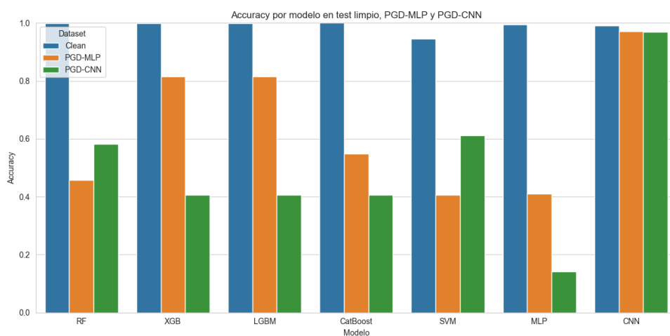
Figura 65. Accuracy-PGD-IOT-23
