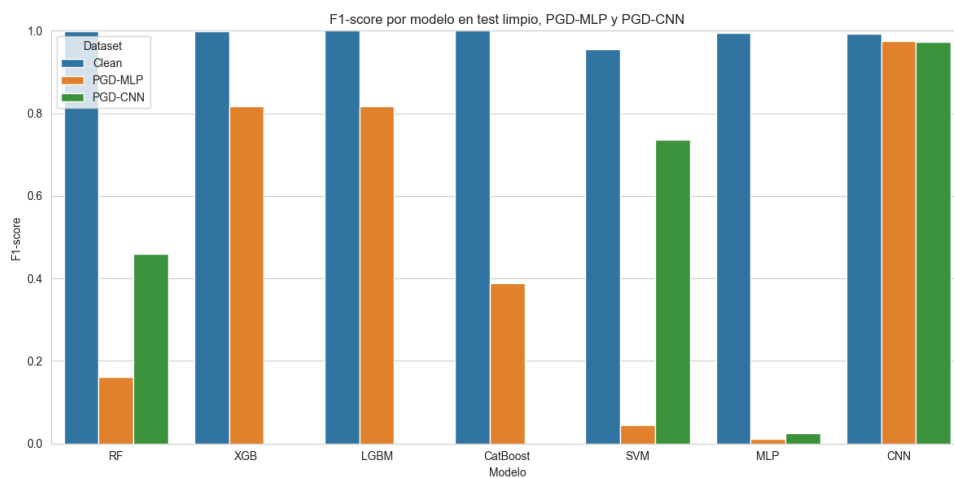
Figura 64. F1-PGD-IOT-23
