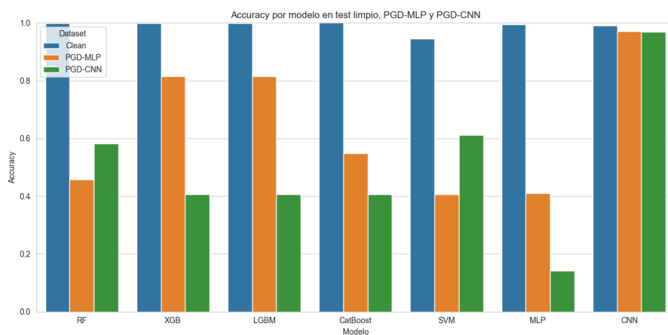
Figura 2.53. Accuracy-PGD-IOT-23
