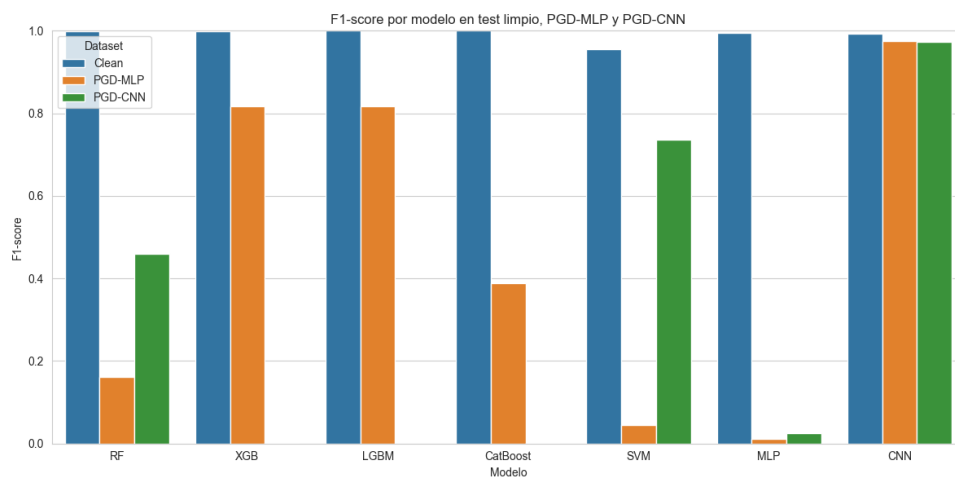
Figura 2.52. F1-PGD-IOT-23
