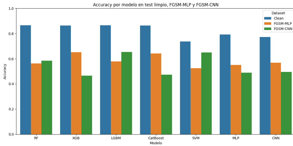
Figura 2.50. Accuracy-FGSM-UNSW-NB15
