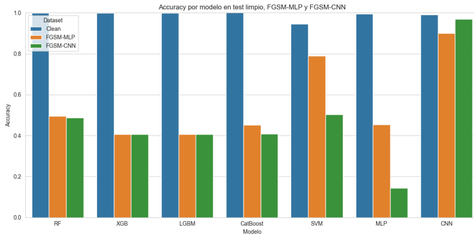
Figura 2.56. Accuracy-FGSM-IOT-23
