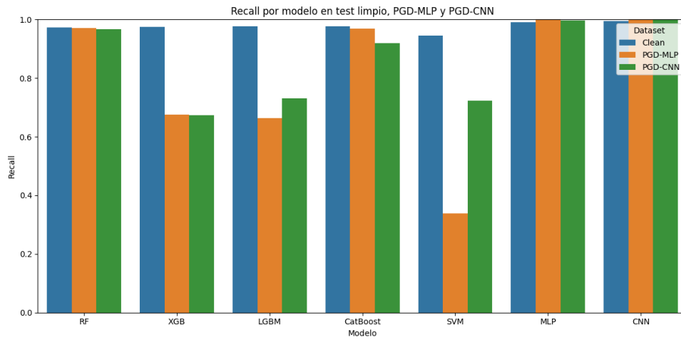
Figura 2.48. Recall-PGD-UNSW-NB15
