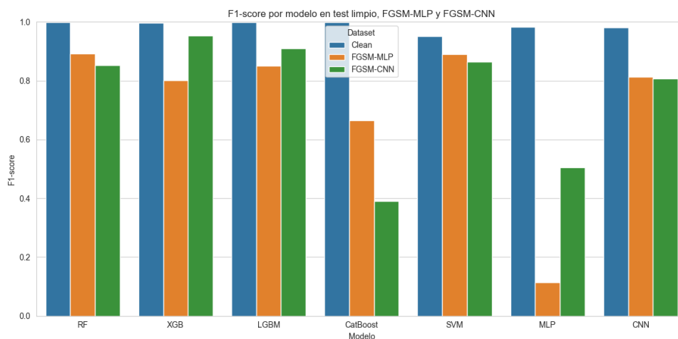
Figura 2.61. F1-FGSM-TON-IOT
