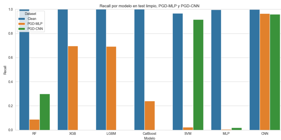
Figura 2.54. Recall-PGD-IOT-23
