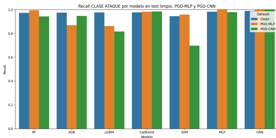
Figura 6.3. Recall-PGD-UNSW-NB15
