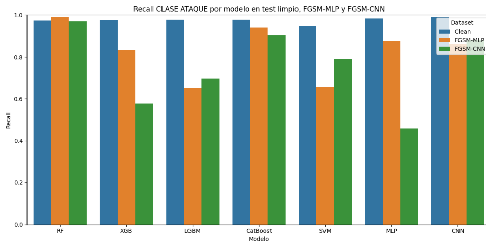
Figura 6.6. Recall-FGSM-UNSW-NB15
