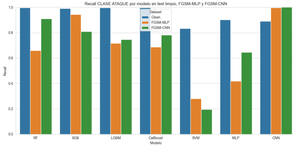
Figura 6.18. Recall-FGSM-TON-IOT
