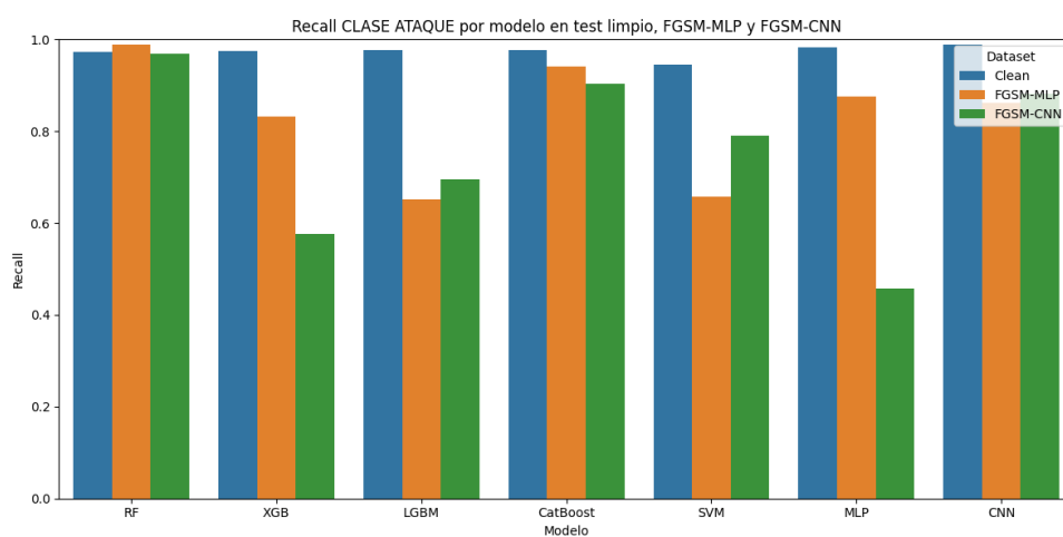
Figura 6.6. Recall-FGSM-UNSW-NB15
