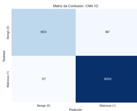
Figura 5.45. MC - CNN (ToN-IoT)
