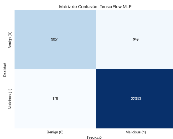
Figura 5.44. MC - MLP (ToN-IoT)
