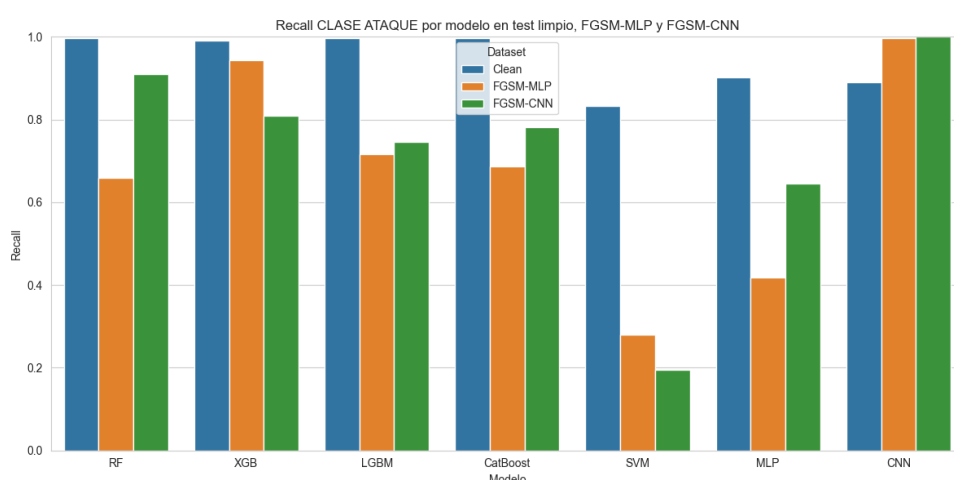
Figura 6.18. Recall-FGSM-TON-IOT
