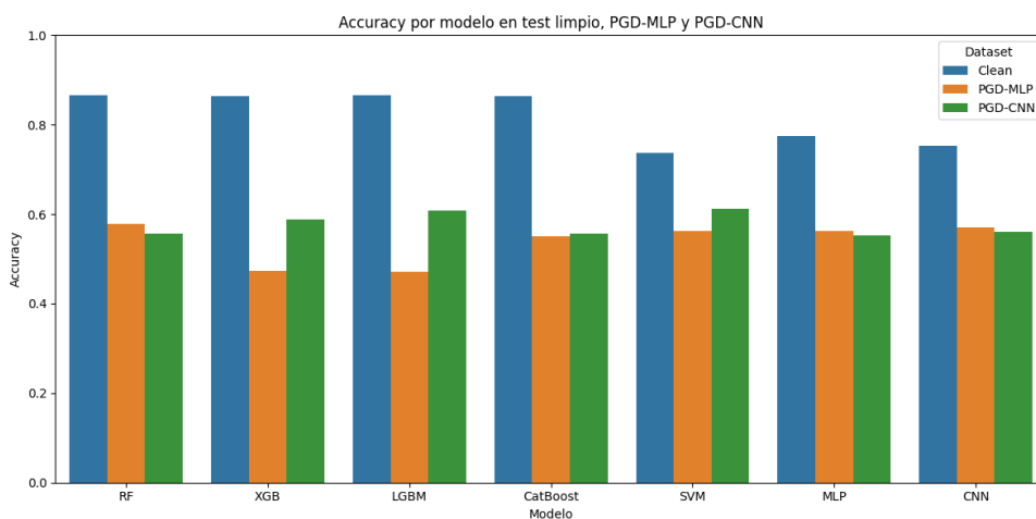
Figura 2.47. Accuracy-PGD-UNSW-NB15
