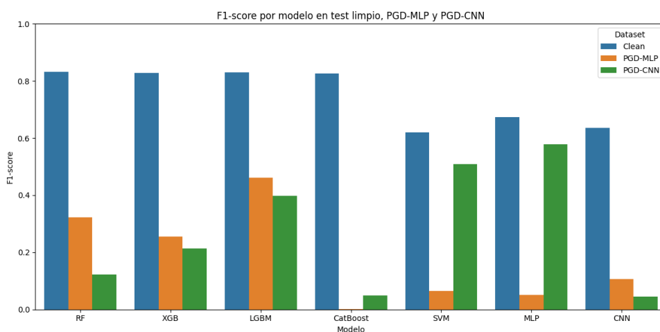
Figura 2.46. F1-PGD-UNSW-NB15
