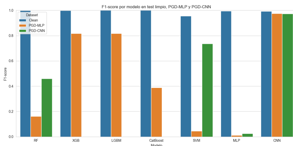
Figura 2.52. F1-PGD-IOT-23
