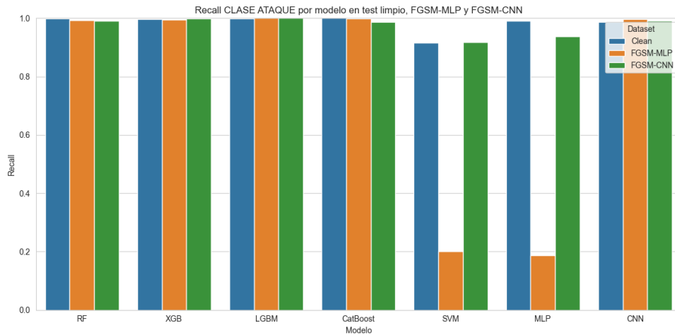
Figura 2.57. Recall-FGSM-IOT-23
