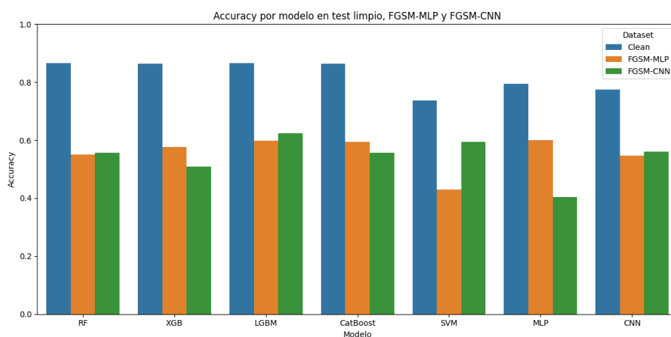
Figura 2.50. Accuracy-FGSM-UNSW-NB15
