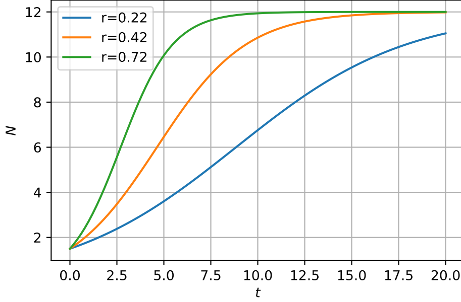
Figure 4.1: Numerical solution of the logistic growth model
