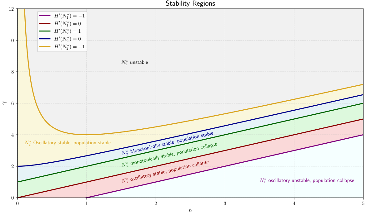
Figure 2.14: Stability regions for the harvesting model.
