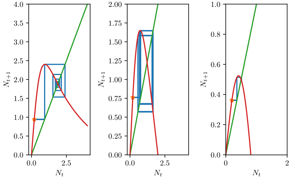
Figure 2.14: Cobweb diagrams for different values of h .
