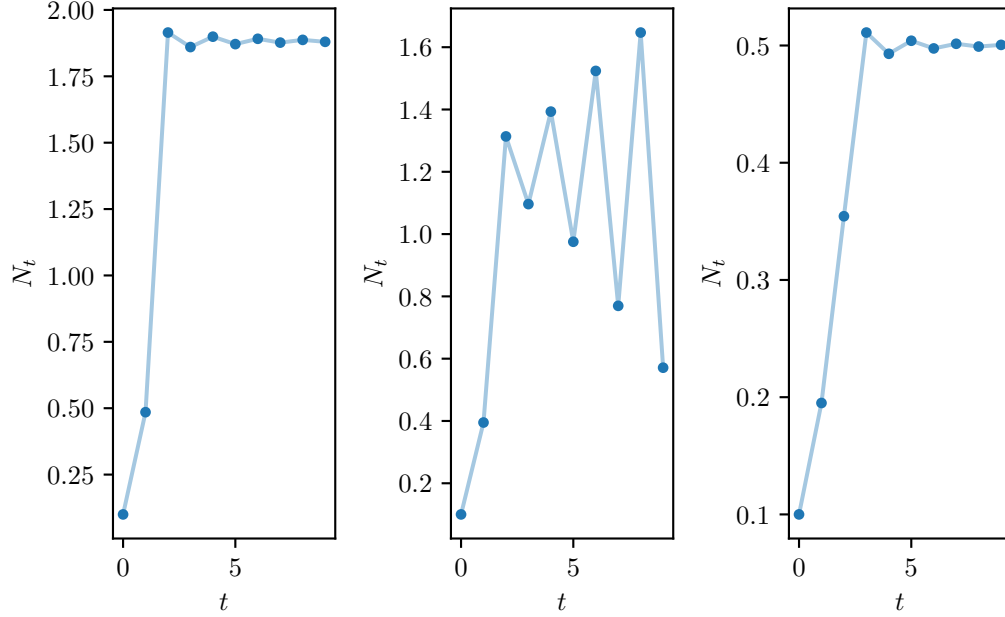
Figure 2.11: Time series solution for different values of h .
