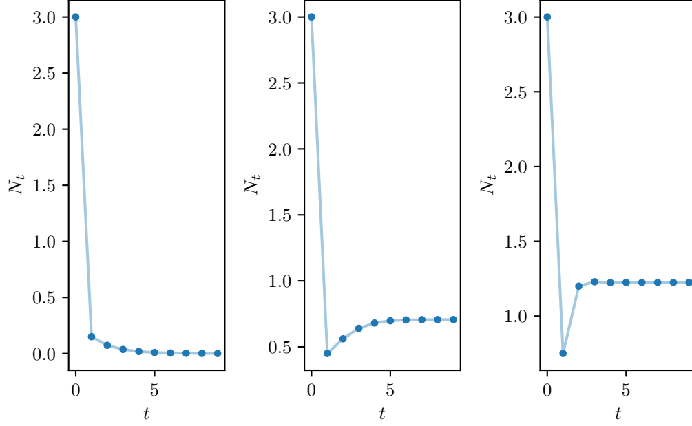
Figure 2.7: Time series solution for (a) \gamma=0.5 and (b) \gamma=1.5 and (c) \gamma=10.5 .
