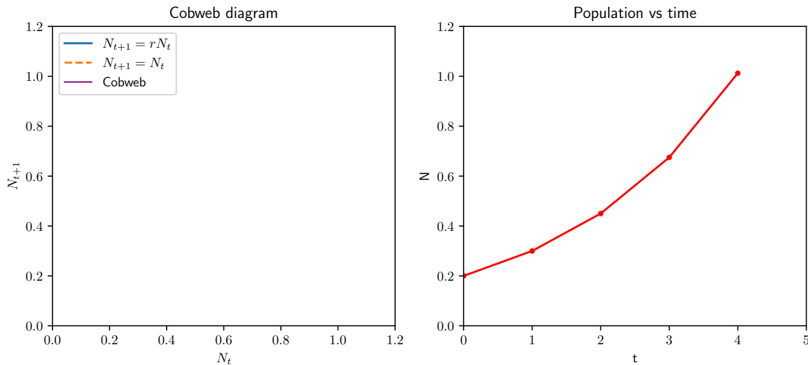
Figure 2.5: Animation of a cobweb diagram for the Malthusian model with N_0 = 0.2 and r = 1.5 .
