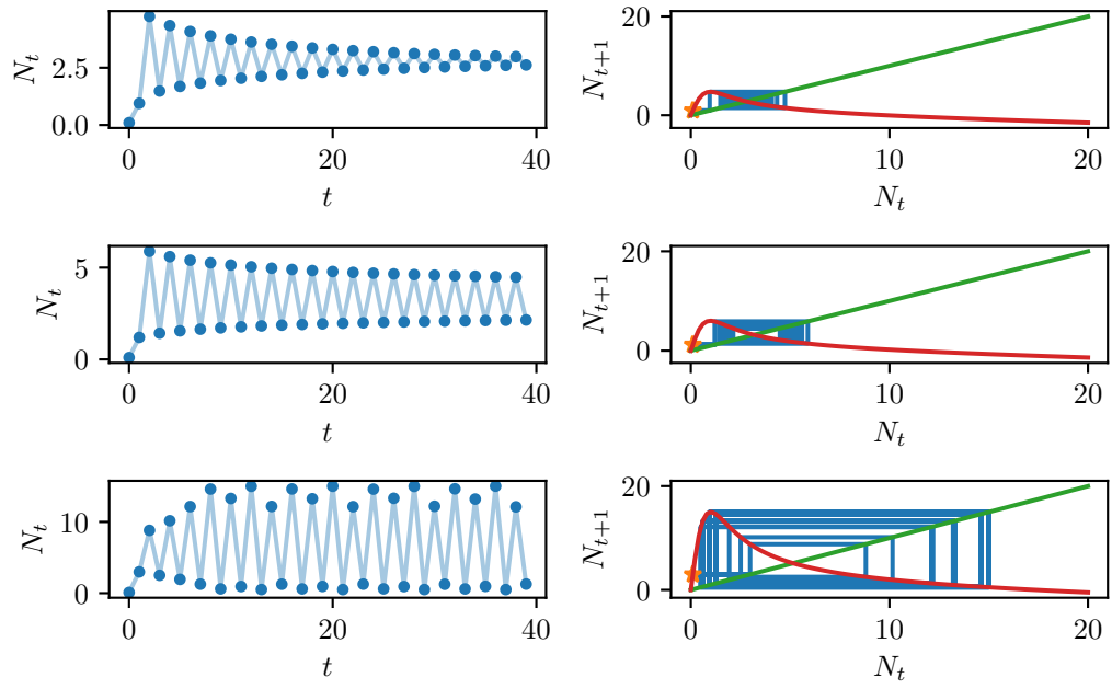
Figure 2.15: Transition from period 2 to period 4 solutions in the harvesting model
