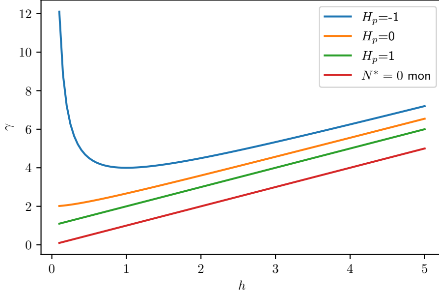
Figure 2.13: Stability regions for the harvesting model.
