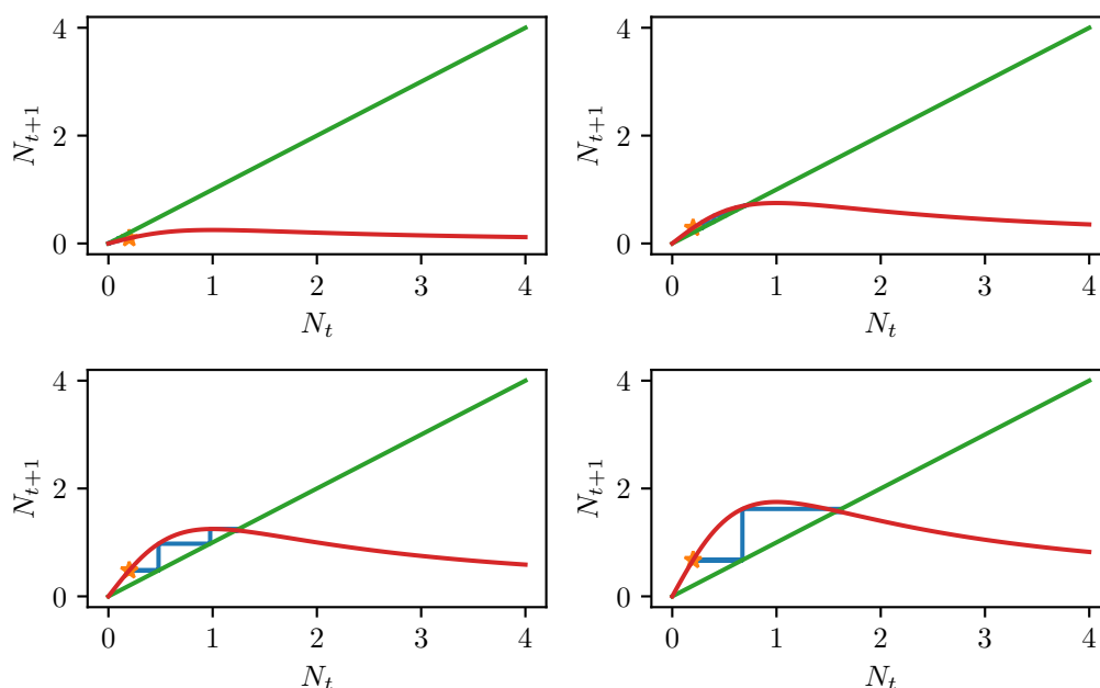
Figure 2.9: Cobweb diagrams for different values of \gamma .
