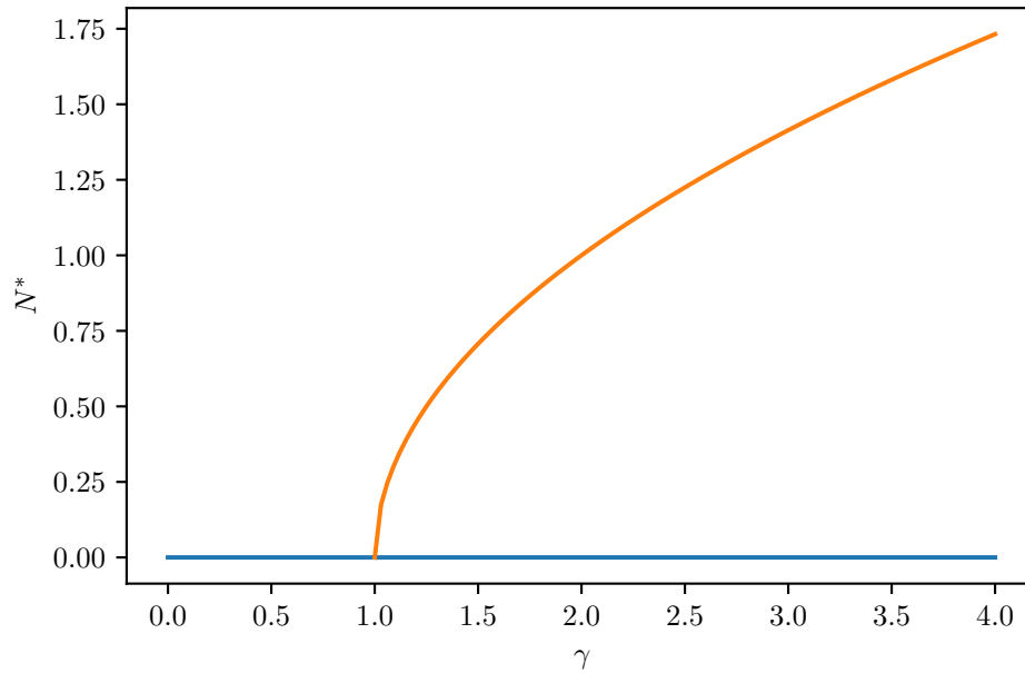
Figure 2.10: A bifurcation diagram.
