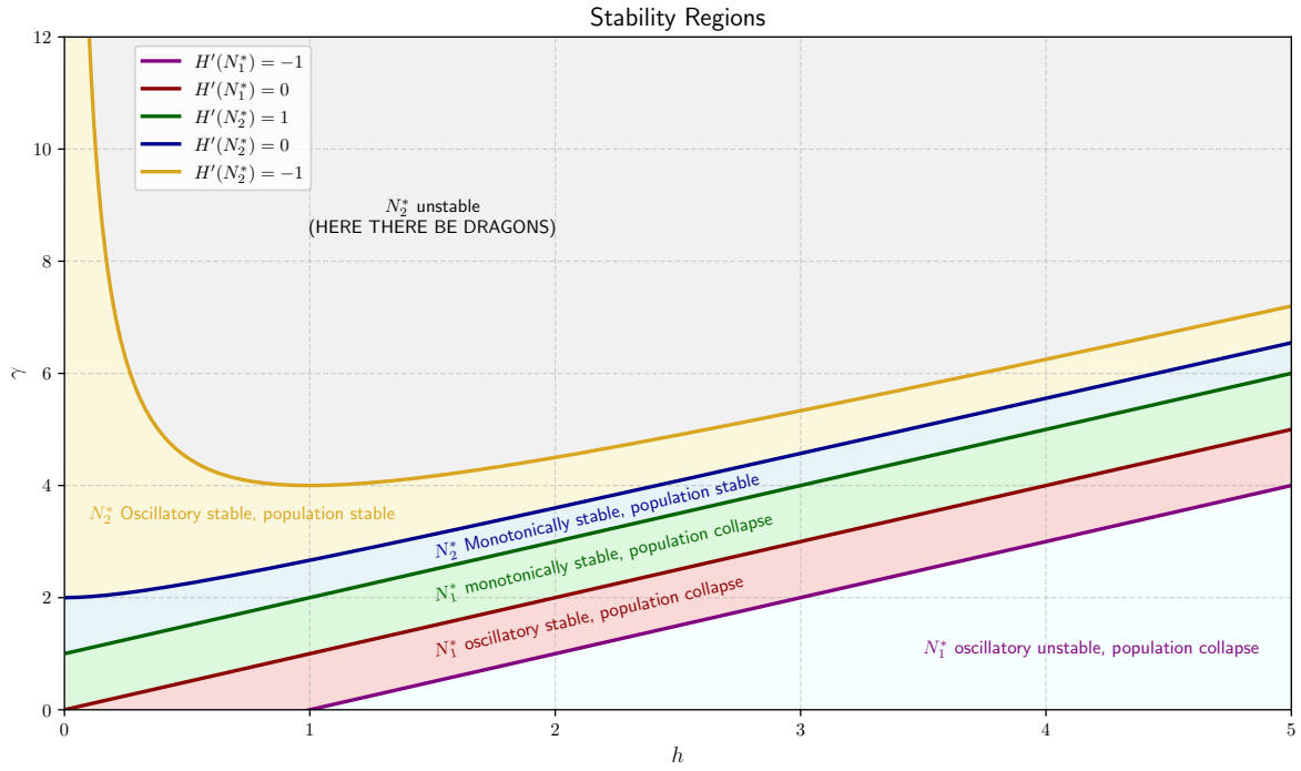
Figure 2.14: Stability regions from studying the linear stability of the fixed points of the harvesting model. This is not enough to understand population stability/collapse for the grey region!
