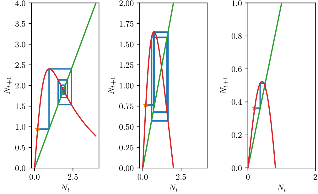
Figure 2.15: Cobweb diagrams for different values of h .
